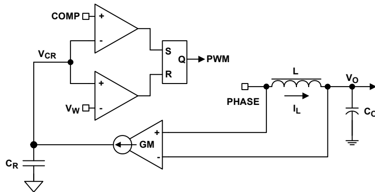
Figure 25. R3 Modulator
