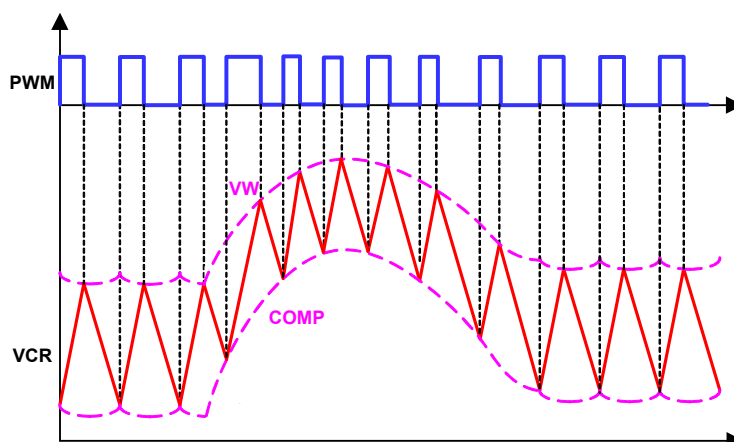
Figure 27. R3 Modulator Operation Principles In Dynamic Response
