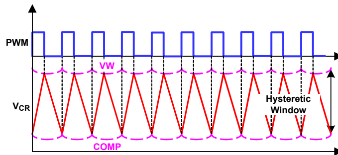
Figure 26. R3 Modulator Operation Principles In Steady State
