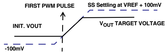
FIGURE 23. SOFT-START WITH V_{OUT} < \text{TARGET VOLTAGE}
