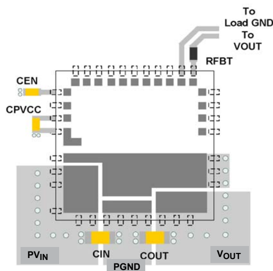
FIGURE 28. RECOMMENDED LAYOUT
