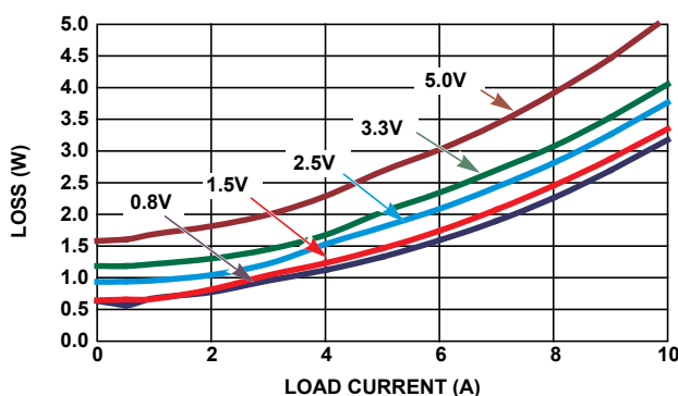
FIGURE 31. POWER LOSS vs LOAD CURRENT (12V IN )
