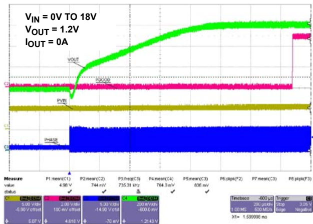
FIGURE 20. 50% PRE-BIAS START-UP
