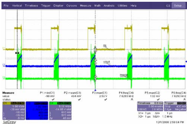
FIGURE 19. OVERCURRENT PROTECTION
