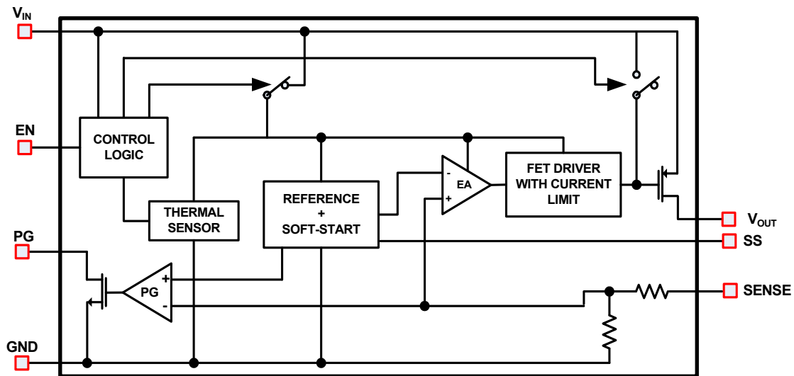
FIGURE 3. BLOCK DIAGRAM
