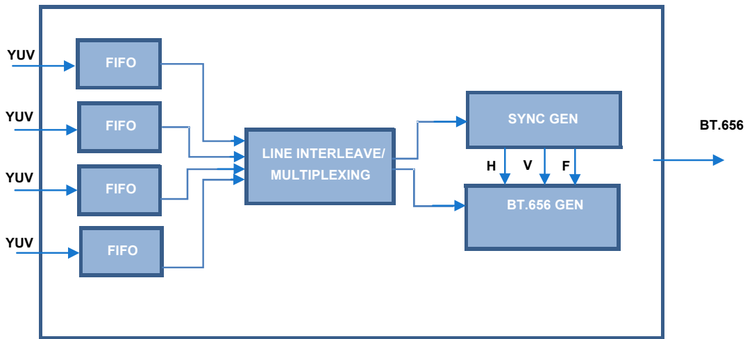
FIGURE 16. ISL79988 - BT.656 LINE-INTERLEAVED OUTPUT
