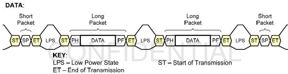
FIGURE 19. SHORT AND LONG PACKETS
