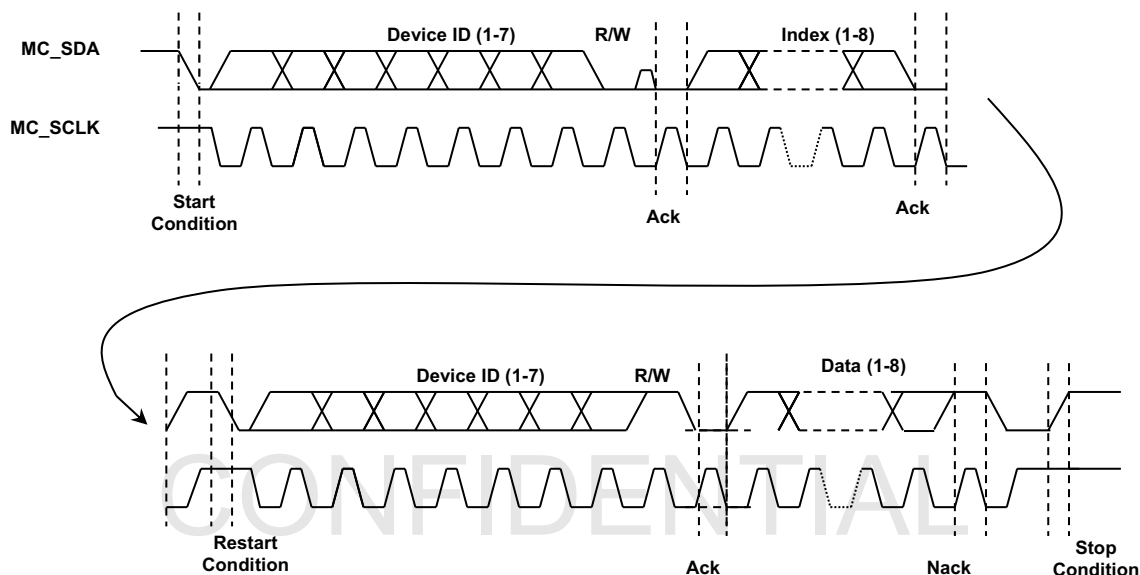
FIGURE 5. ONE COMPLETE REGISTER READ SEQUENCE USING THE SERIAL BUS INTERFACE
