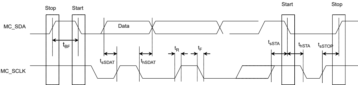
FIGURE 6. SERIAL BUS INTERFACE TIMING
