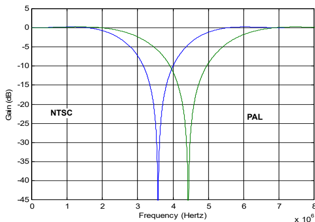
FIGURE 12. CHARACTERISTICS OF LUMINANCE NOTCH FILTER FOR PAL
