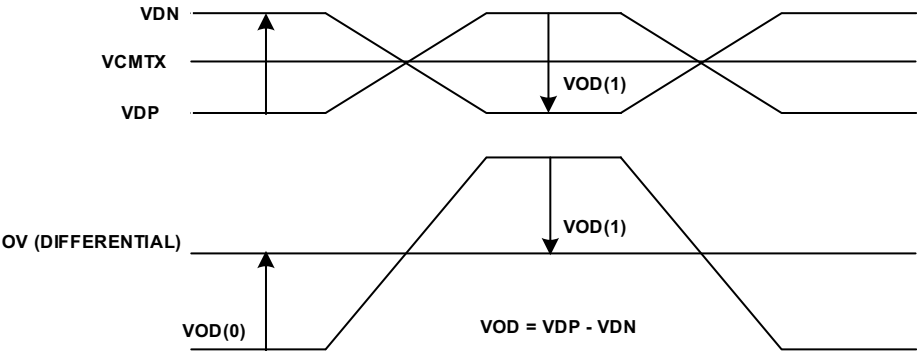
FIGURE 7. ISL79987 MIPI LOW POWER AC TIMING
