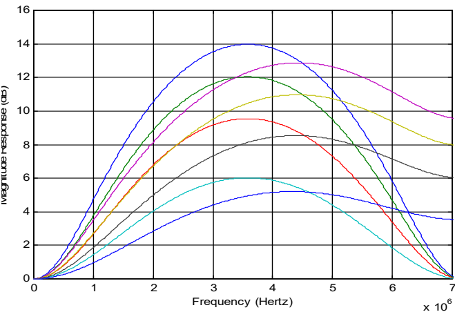
FIGURE 15. CHARACTERISTIC OF THE LUMINANCE PEAKING FILTER
