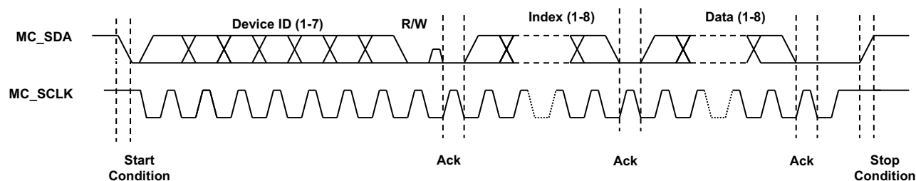
FIGURE 4. ONE COMPLETE REGISTER WRITE SEQUENCE USING THE SERIAL BUS INTERFACE
