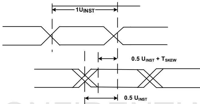
FIGURE 8. ISL79987 MIPI SPEED POWER AC TIMING
