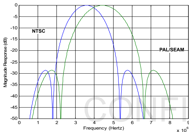
FIGURE 13. CHROMA BAND-PASS FILTER CURVES
