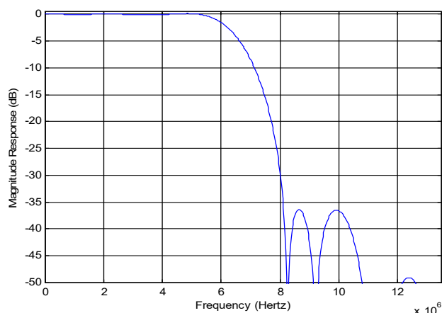
FIGURE 11. FREQUENCY RESPONSE OF THE DECIMATION FILTER
