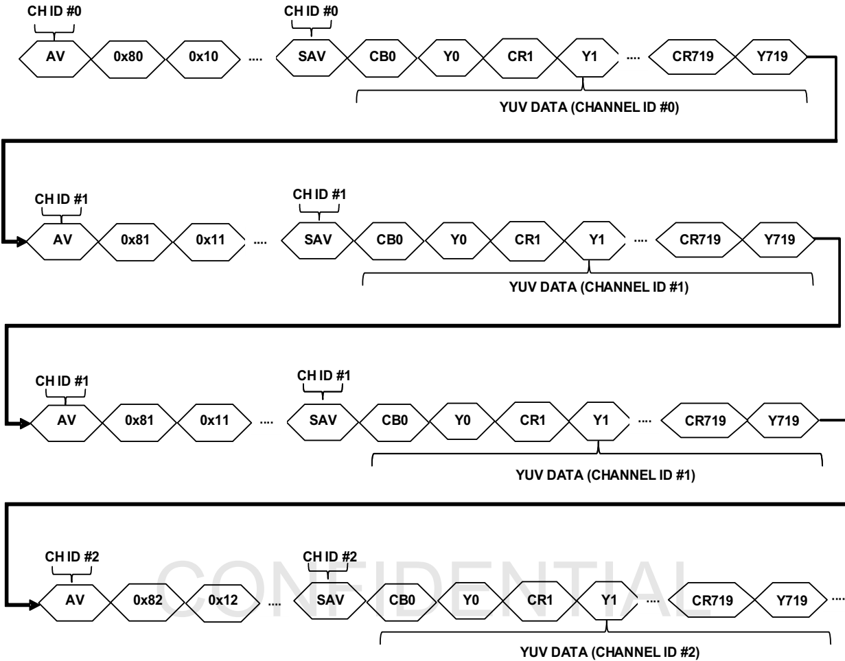
FIGURE 17. BT.656 INTERLEAVED DATA TRANSMISSION WITH CHANNEL ID
