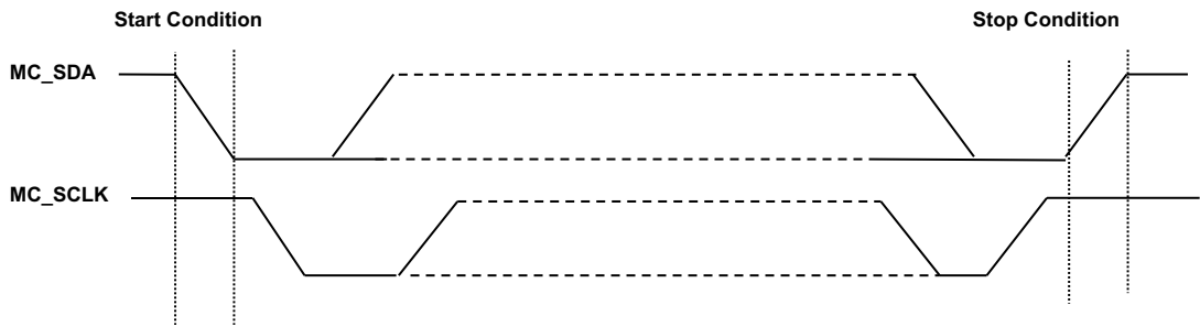
FIGURE 3. DEFINITION OF THE SERIAL BUS INTERFACE BUS START AND STOP
