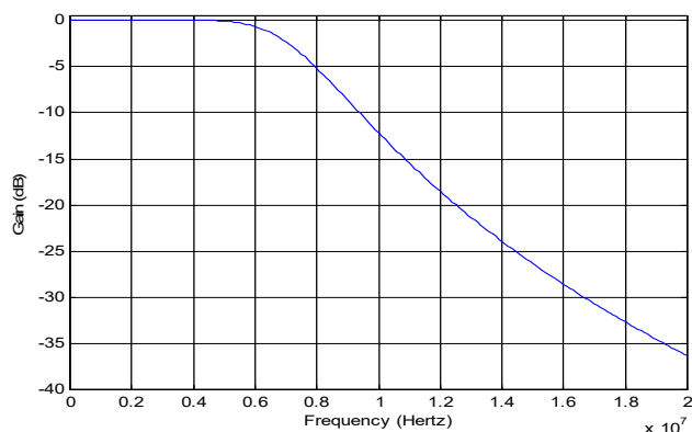
FIGURE 10. FREQUENCY RESPONSE OF THE ANTI-ALIASING FILTER
