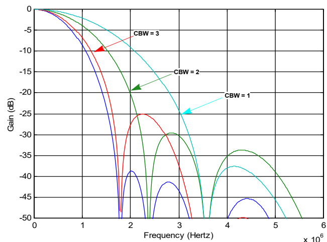
FIGURE 14. CHROMINANCE LOW-PASS FILTER CURVES
