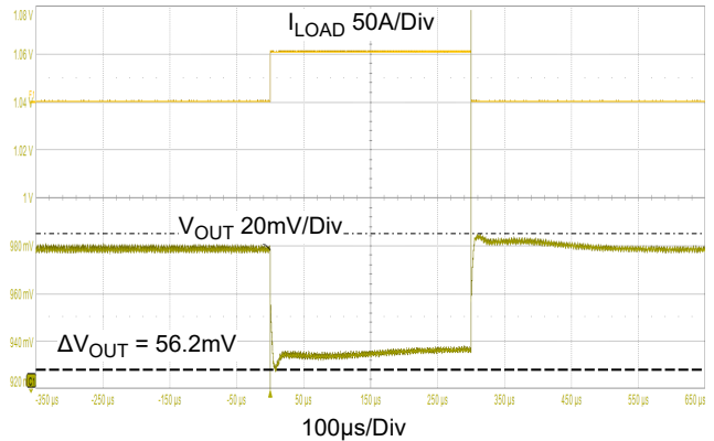
Figure 26. Load Transient Response ( P_{VIN} = V_{DD} = 12V , R_{DROOP} = 604\Omega )
