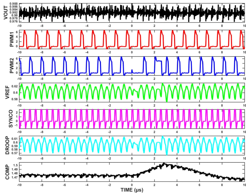
Figure 75. f_{\text{SW}} = 1\text{MHz} , trigger V_{\text{OUT}} \pm 20\text{mV}
