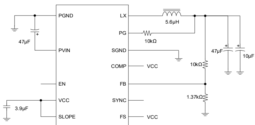
Figure 2. Internal Compensation Application Diagram for 12V to 5V, 500kHz
