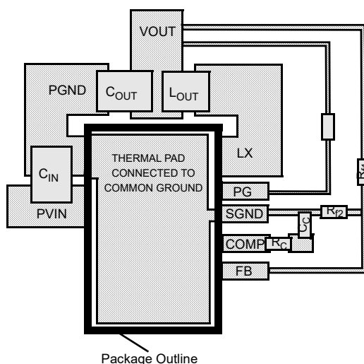
Figure 58. Layout Component Placement Suggestion
