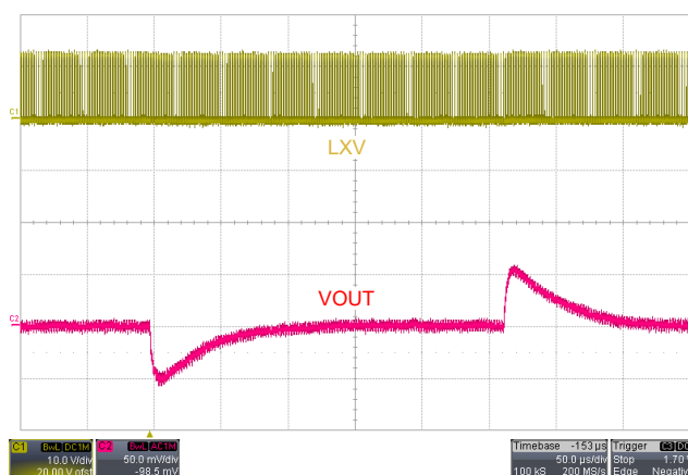
Figure 52. 12V_{IN} , 3.3V_{OUT} , 500kHz, 2A Load Transient (Internal Compensation), L_{OUT} = 4.7\mu H , C_{OUT} = 144\mu F
