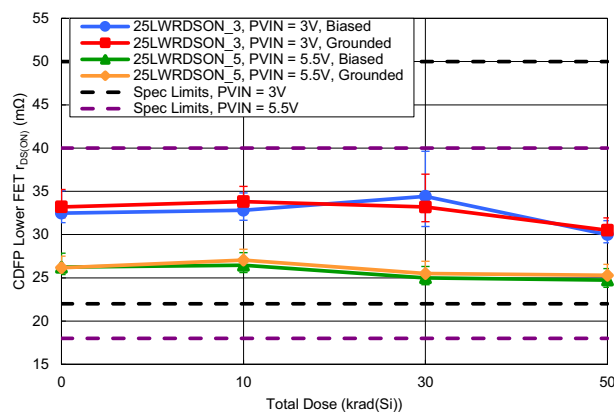
Figure 66. CDFP Lower FET r_{DS(ON)}
