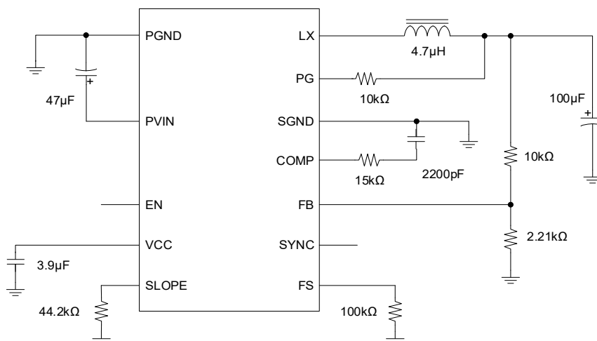
Figure 54. External Compensation Application Diagram for 12V to 3.3V, 500kHz
