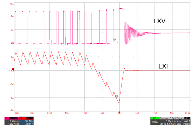
Figure 38. Negative Overcurrent Protection, Negative Overcurrent Event and Shutdown
