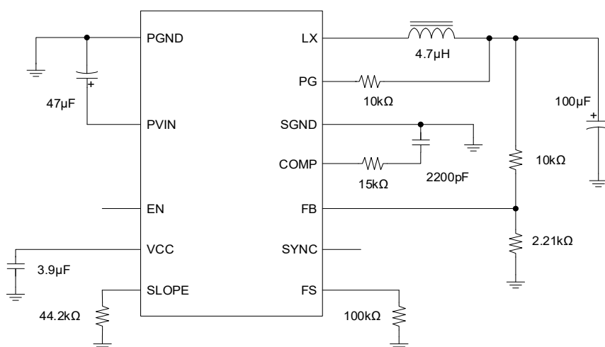
Figure 1. External Compensation Application Diagram for 12V to 3.3V, 500kHz
