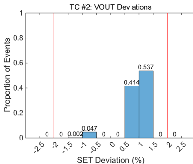
Figure 67. Test Condition #2: VOUT Deviation Size of SETs
