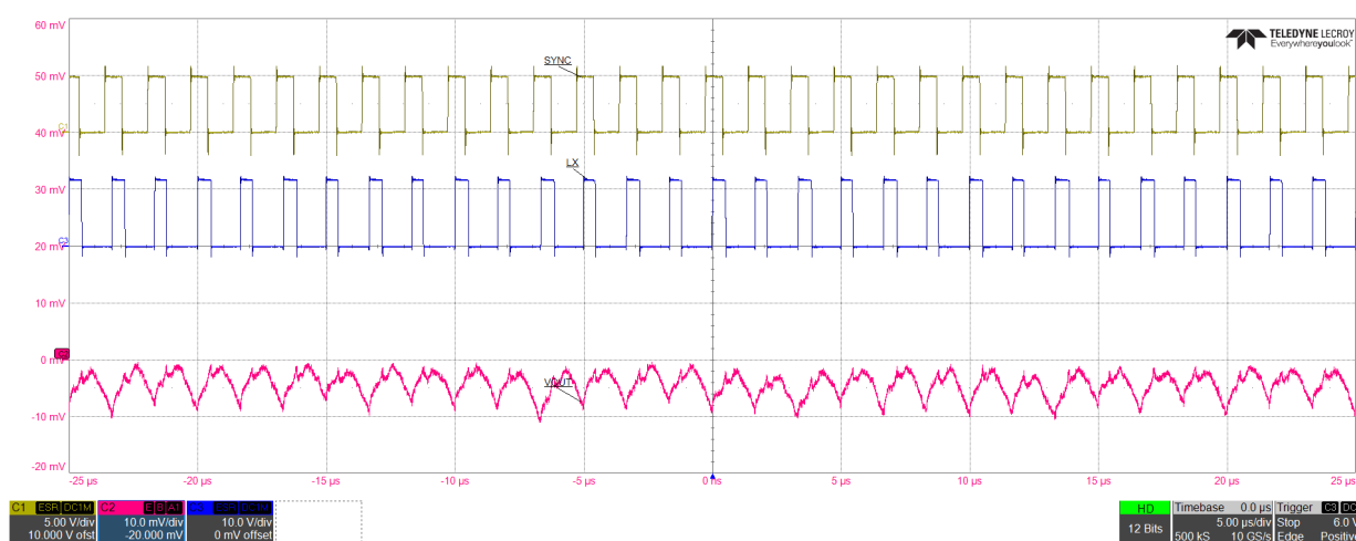
Figure 55. Output Voltage Ripple with External Clock ( V_{IN} = 12V , V_{OUT} = 3.3V , I_{OUT} = 3A , R1 = 221\Omega , R2 = 1k\Omega , SYNC_{freq} = 600kHz )
