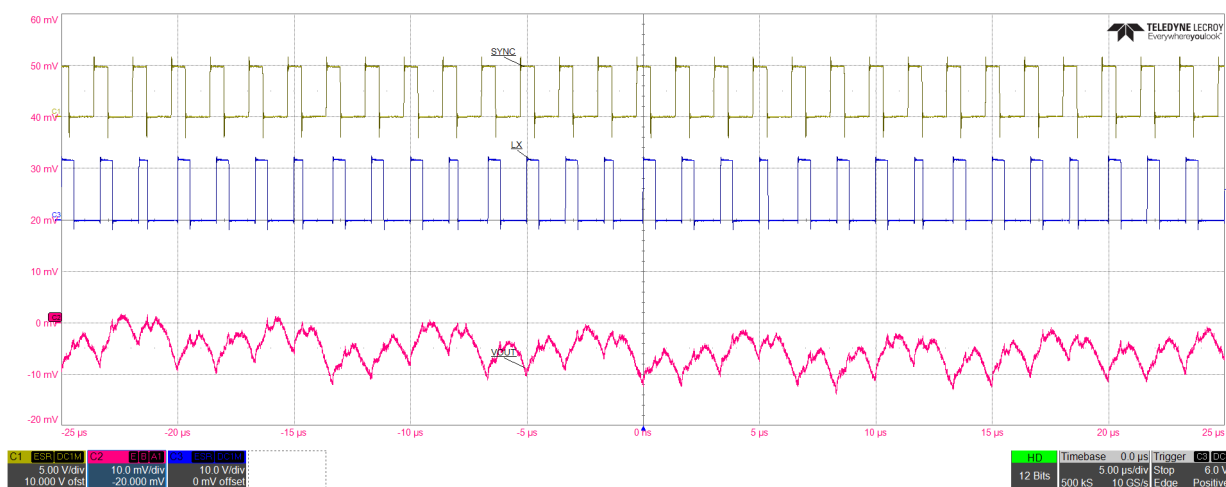
Figure 56. Output Voltage Ripple with External Clock ( V_{IN} = 12V , V_{OUT} = 3.3V , I_{OUT} = 3A , R1 = 2.21k\Omega , R2 = 10k\Omega , SYNC_{freq} = 600kHz )
