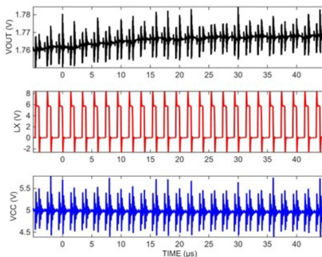
Figure 68. Typical SET Capture
