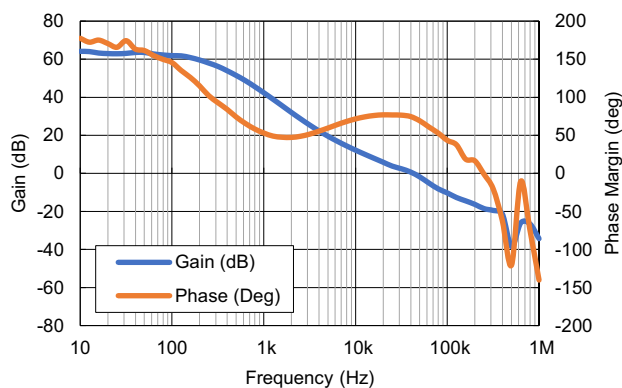
Figure 50. Internal Comp Gain/Phase BODE Plot, 12V_{IN} , 3.3V_{OUT} , 500kHz , I_{OUT} = 1.5A L_{OUT} = 4.7\mu H , C_{OUT} = 144\mu F
