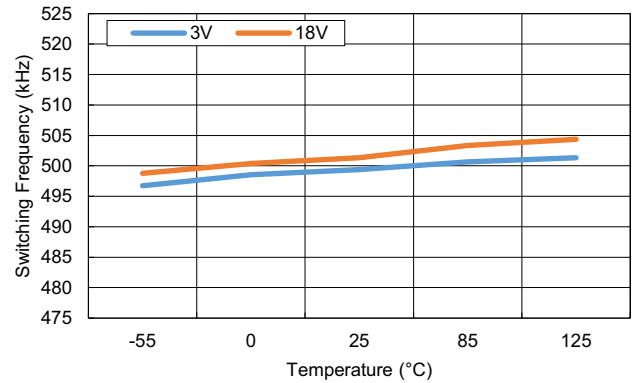
Figure 12. 100kΩ External 500kHz vs Temperature
