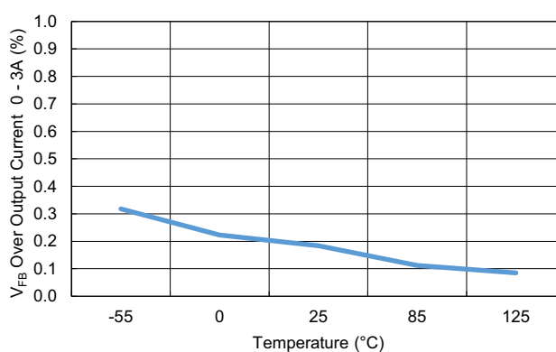
Figure 26. V_{FB} Over Output Current vs Temperature
