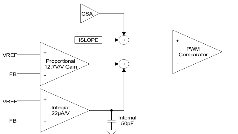
Figure 53. Internal Error Amplifier Block Diagram
