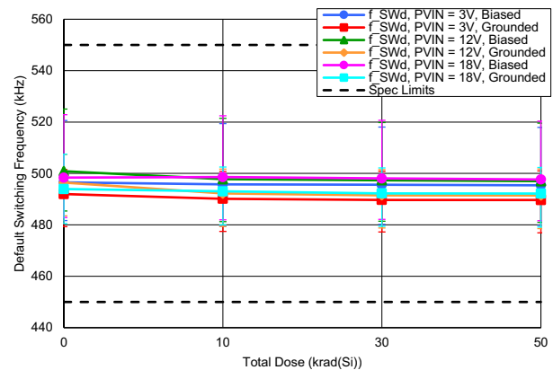
Figure 61. Default Switching Frequency
