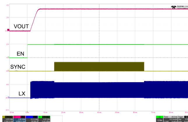
Figure 43. SYNC Turn-On after LX Switching
