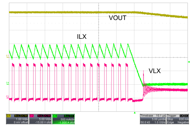
Figure 31. Overcurrent Protection Function
