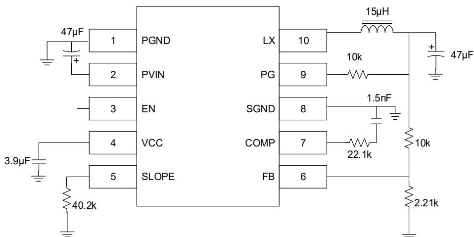
Figure 46. Typical Application
