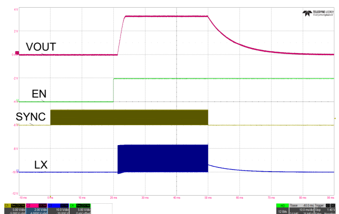
Figure 44. SYNC Turn-On before LX Switching
