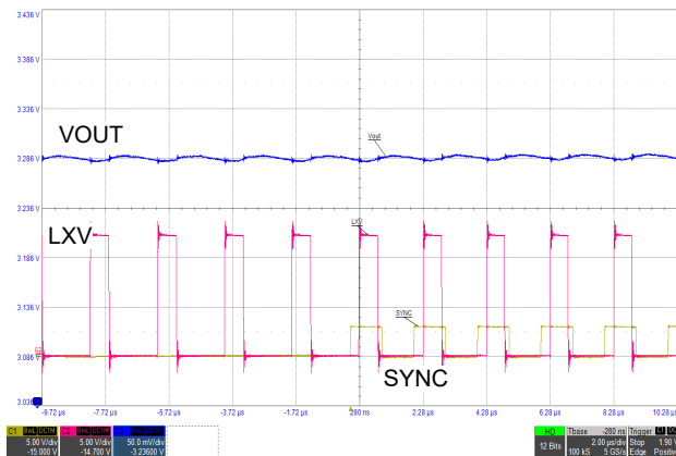
Figure 41. 500kHz SYNC Input Start
