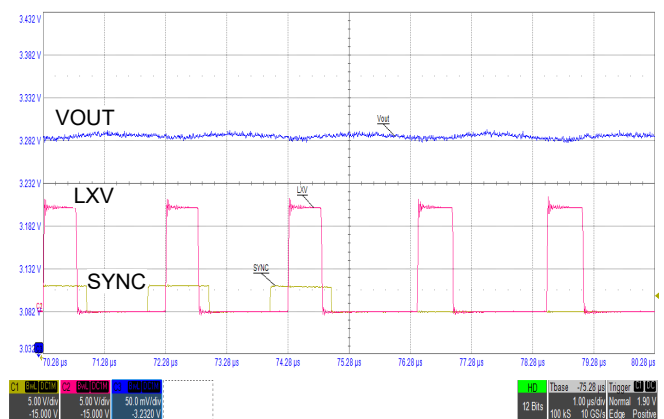
Figure 42. 500kHz SYNC Input Stop
