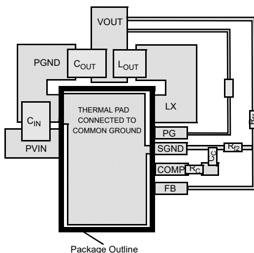
Figure 48. Layout Component Placement Suggestion
