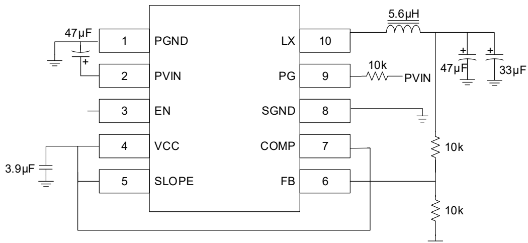
Figure 2. Internal Compensation Application Diagram for 5V to 1.2V
