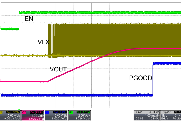
Figure 30. ENABLE to LX and VOUT to PGOOD
