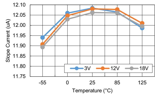
Figure 27. SLOPE Current vs Temperature
