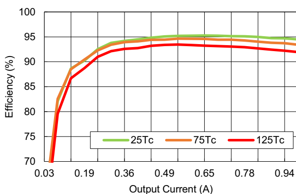
Figure 36. Efficiency 12V IN to 5V OUT vs Case Temp
