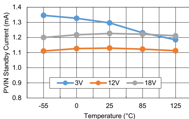
Figure 6. Standby Current vs Temperature
