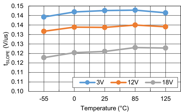
Figure 28. Slope Ramp Rate vs Temperature
