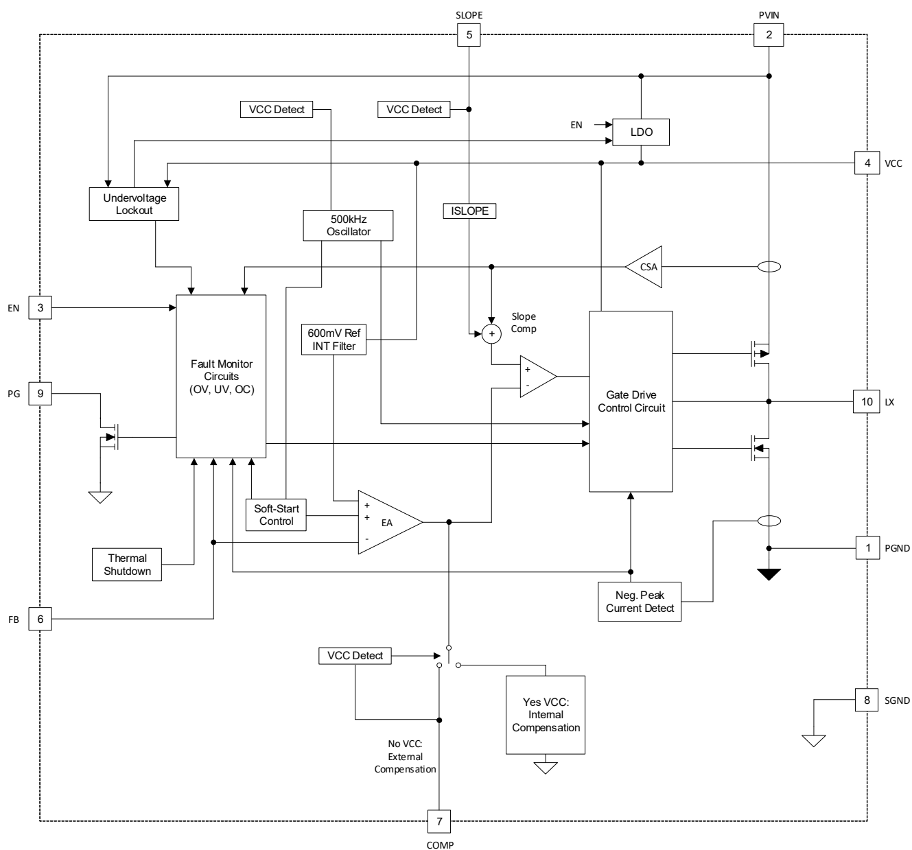
Figure 3. Block Diagram
