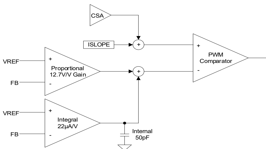
Figure 45. Internal Error Amplifier Block Diagram
