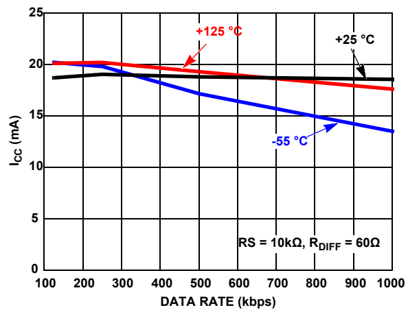
Figure 25. Supply Current vs Medium Data Rate vs Temperature
