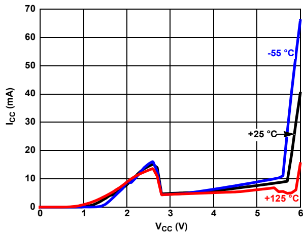
Figure 44. Supply Current vs Supply Voltage vs Temperature
