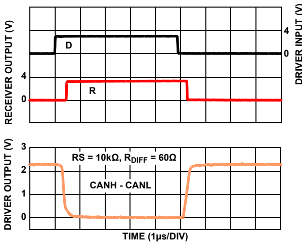
Figure 46. Medium Driver and Receiver Waveforms
