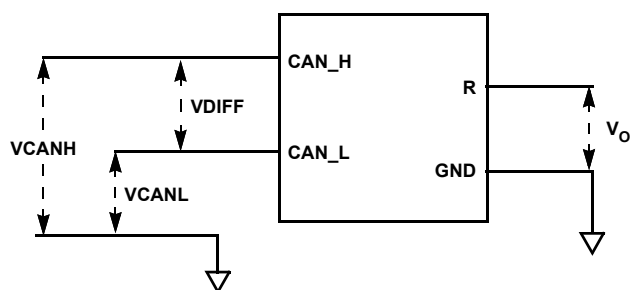
Figure 15. Receiver Voltage Definitions
