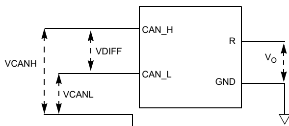
Figure 16. Receiver Voltage Definitions
