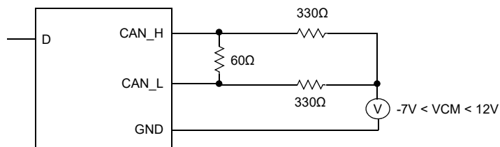
Figure 13. Driver Common-Mode Circuit
