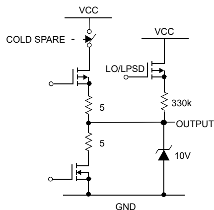
Figure 8. R Output
