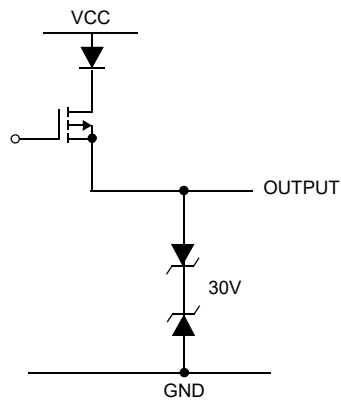
Figure 5. CANH Output
