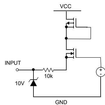
Figure 9. RS Input
