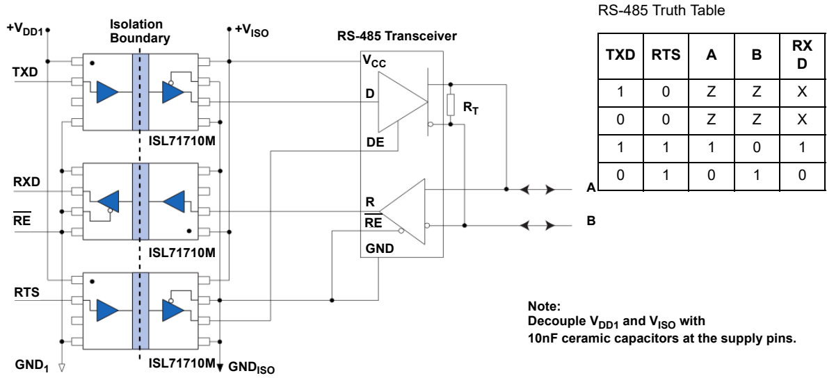
Figure 3. RS-485 Multi-Chip Isolated Transceiver Application Schematic
