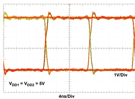
Figure 12. 75Mbps Eye Diagram
