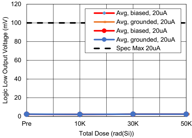
Figure 34. 5V Logic Low Output Voltage vs TID, 20uA
