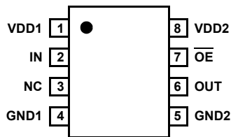
Figure 5. Pin Assignments - Top View
