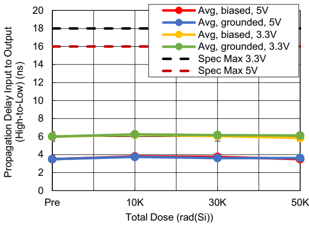
Figure 36. Propagation Delay (High-to-Low) vs TID
