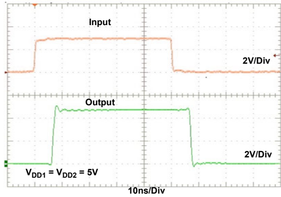
Figure 8. 10MHz Input and Output Waveforms
