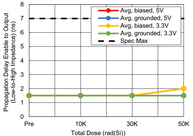
Figure 39. Propagation Delay EN (Low-to-High Z) vs TID
