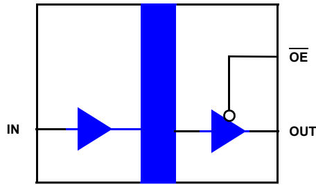
Figure 4. ISL71710M Block Diagram
