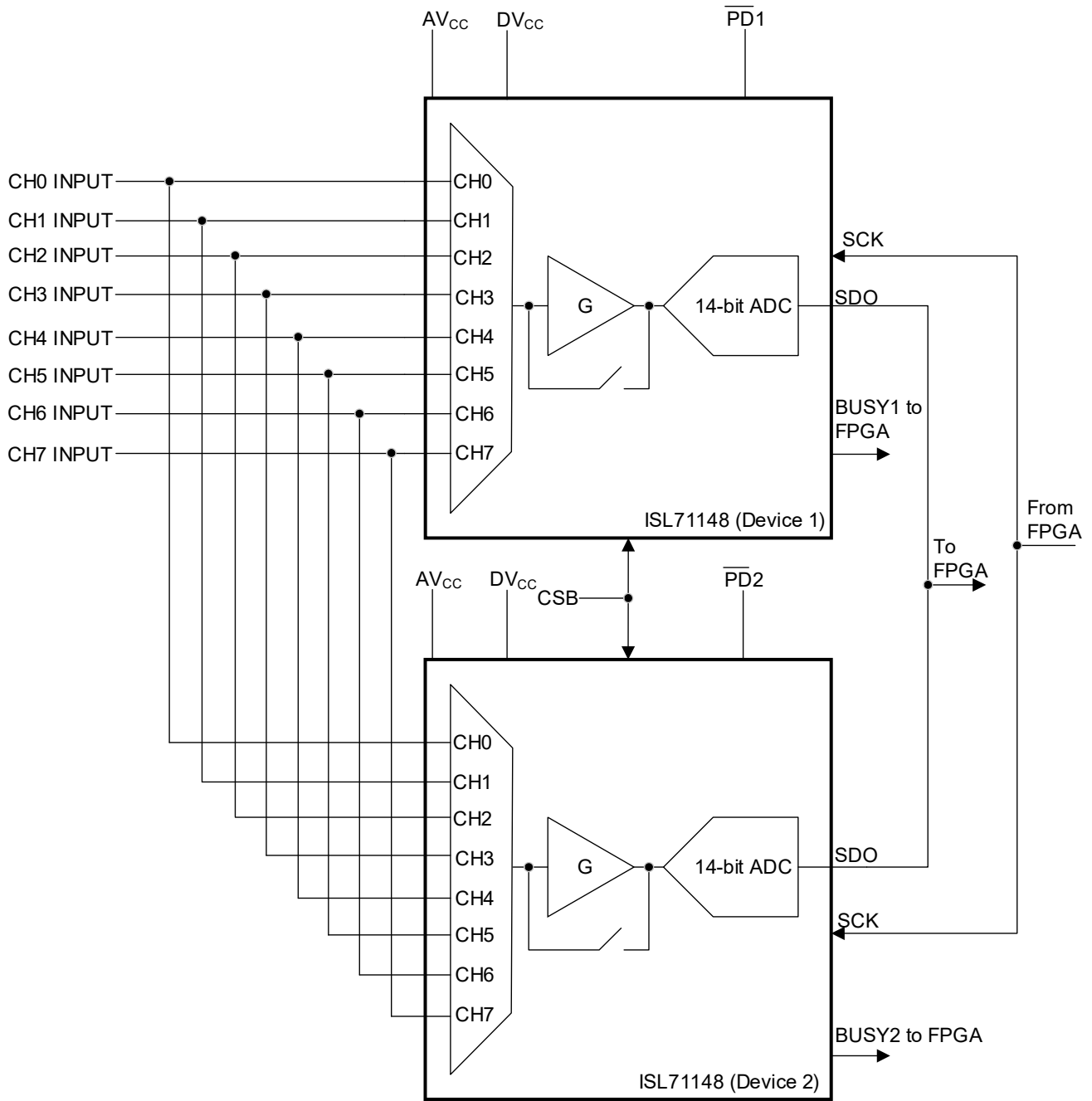
Figure 129. Cold Sparing Example Circuit
