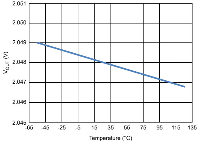
Figure 25. Simulated (Worst Case) V_{OUT} vs Temperature
