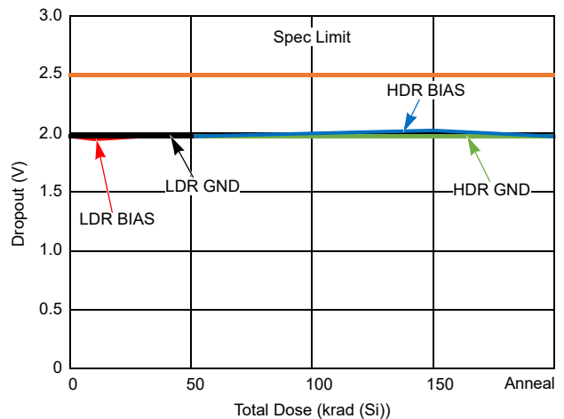
Figure 11. Dropout Shift
