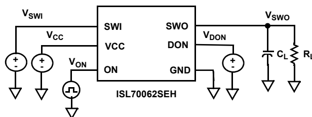
Figure 10. Timing Test Circuit
