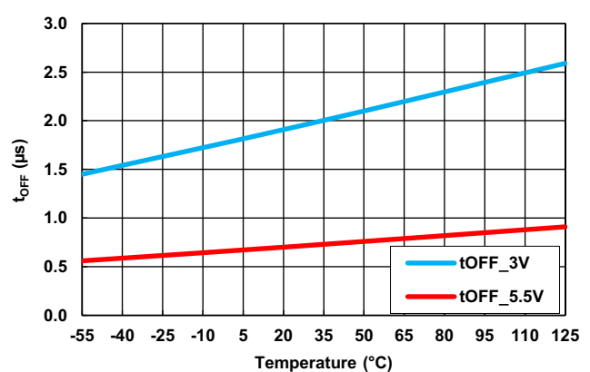
Figure 28. t_{OFF} vs Temperature vs V_{CC}
