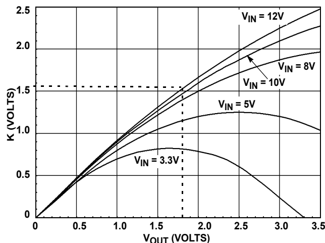
FIGURE 5. EXPANSION OF FIGURE 4 FOR V_{OUT} < 3.5\text{V}
