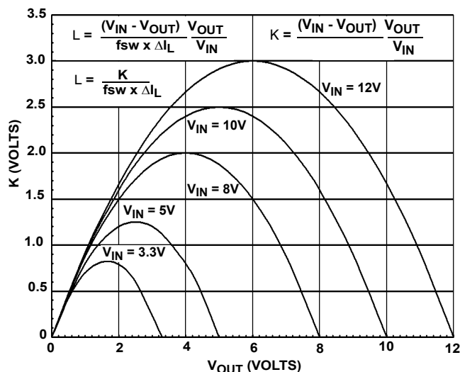
FIGURE 4. "K" AS A FUNCTION OF V_{OUT} FOR FAMILIES OF V_{IN}
