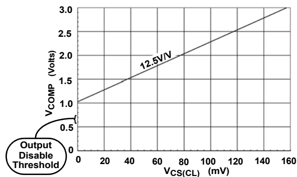
FIGURE 2. CURRENT COMPARATOR THRESHOLD VOLTAGE AS A FUNCTION OF VCOMP
