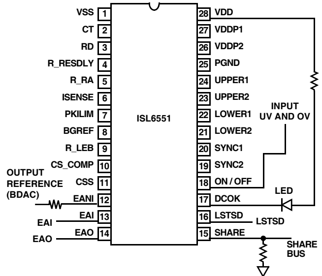
FIGURE 21. ISL6551IREC CONTROLLER
