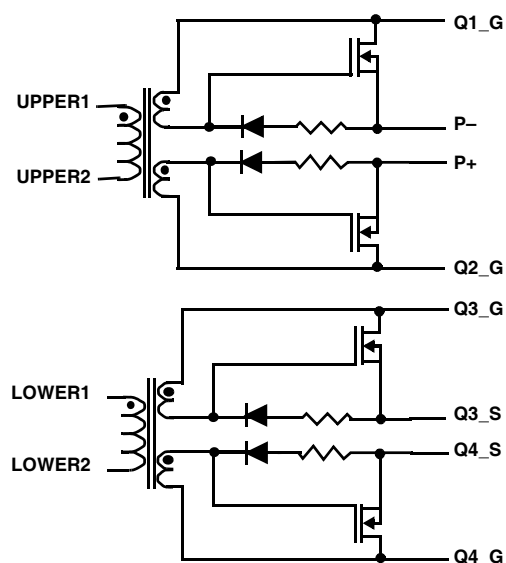
FIGURE 24B. FULL BRIDGE MEDIUM CURRENT DRIVERS
