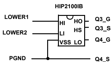
FIGURE 23C. PUSH-PULL PRIMARY CONTROL
