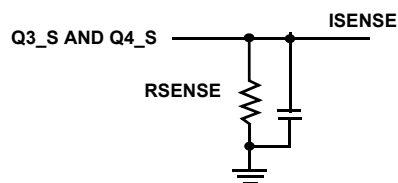
FIGURE 14C. RESISTOR SENSE (PRIMARY CONTROL)
