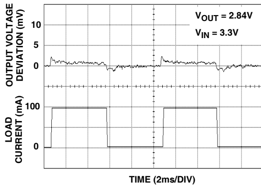
FIGURE 7. LOAD REGULATION RESPONSE ( V_{OUT2} )
