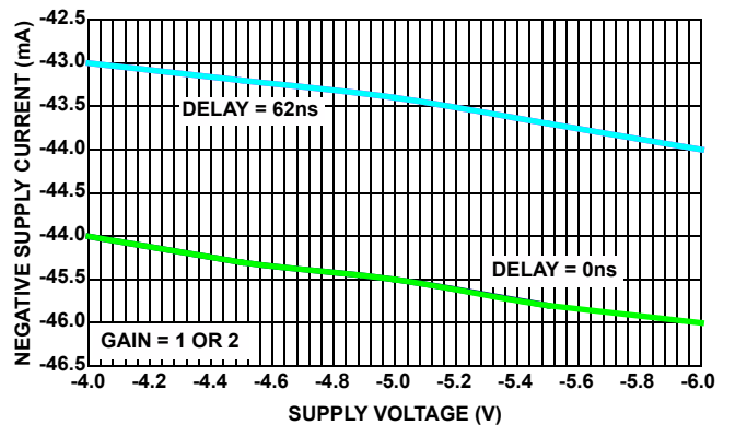
FIGURE 26. ISL59920 I_{SUPPLY-} vs V_{SUPPLY-}
