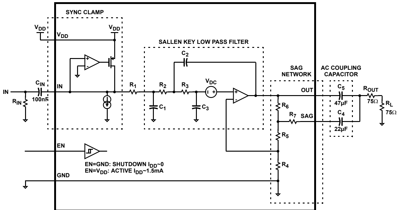
FIGURE 22. BLOCK DIAGRAM
