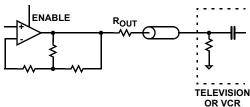
FIGURE 24. DC COUPLE
