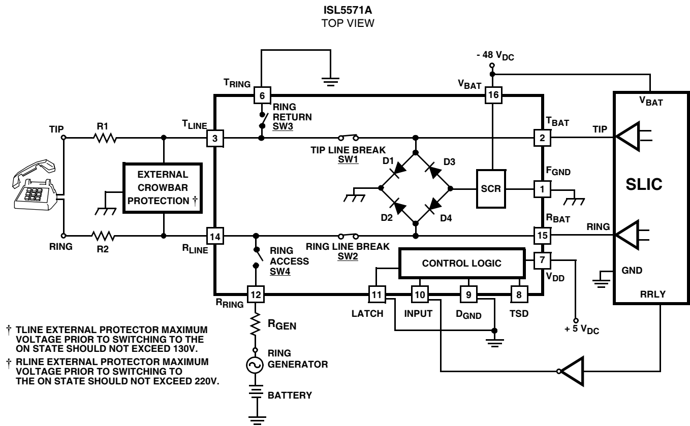
FIGURE 1. APPLICATION CIRCUIT
