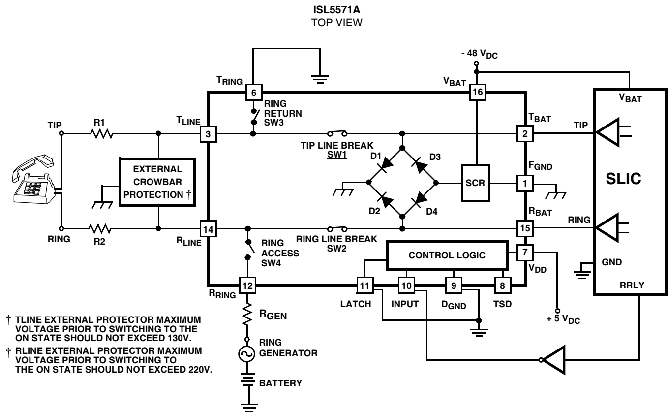
FIGURE 1. APPLICATION CIRCUIT
