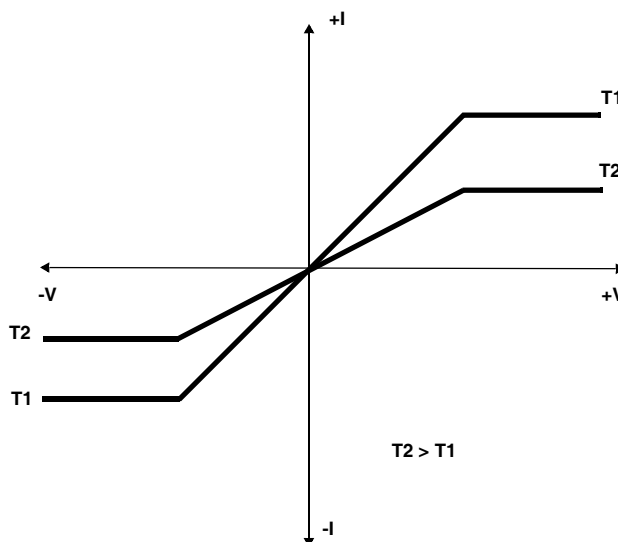
FIGURE 4. EFFECT OF TEMPERATURE ON DC CURRENT LIMIT
