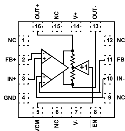
ISL55020 (16 LD QFN) TOP VIEW
