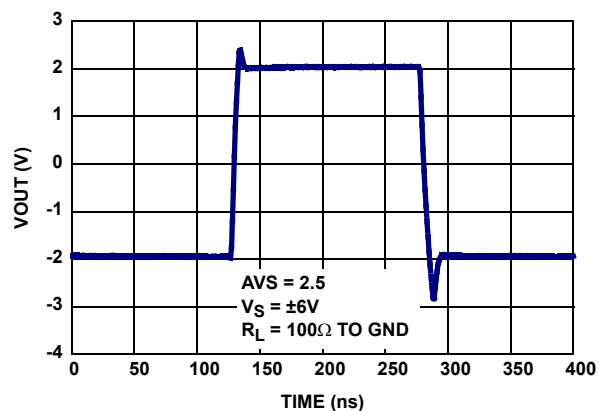
FIGURE 16. LARGE SIGNAL STEP RESPONSE - VCM TO V_{OUT}
