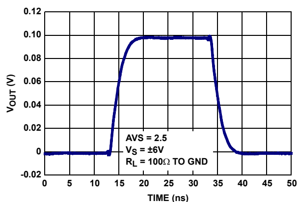
FIGURE 15. SMALL SIGNAL STEP RESPONSE - VCM TO V OUT
