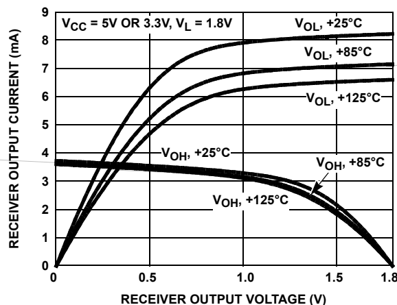
FIGURE 12. RECEIVER OUTPUT CURRENT vs RECEIVER OUTPUT VOLTAGE
