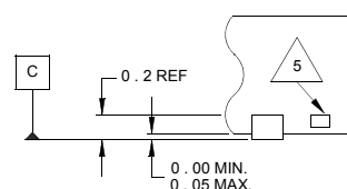
DETAIL "X"
