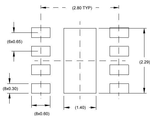
TYPICAL RECOMMENDED LAND PATTERN
