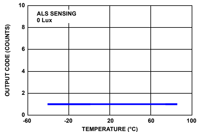
FIGURE 14. OUTPUT CODE FOR 0 LUX vs TEMPERATURE
