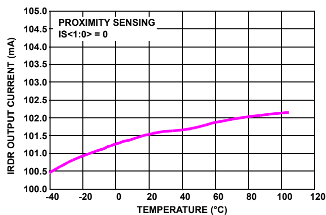
FIGURE 16. OUTPUT CURRENT vs TEMPERATURE IN PROXIMITY SENSING
