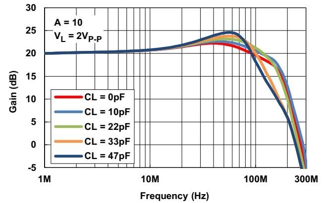
Figure 9. Small Signal Frequency Response vs C_{LOAD}
