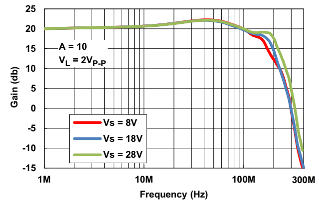
Figure 13. Small Signal Frequency Response vs Supply Voltage
