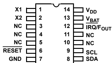
ISL12029, ISL12029A (14 LD TSSOP, SOIC) TOP VIEW
