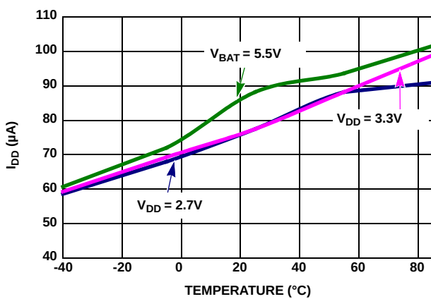
Figure 14. I_{DD} with TSE = 1 vs Temperature
