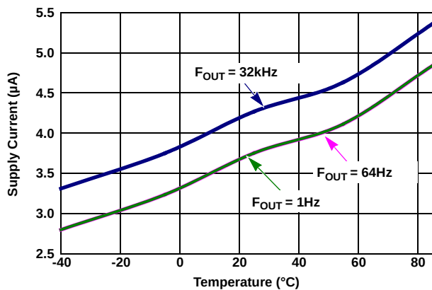
Figure 12. I_{DD} vs Temperature, 3 Different F_{OUT}
