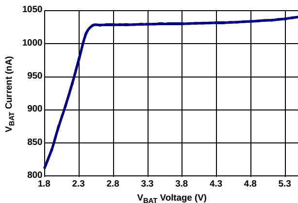
Figure 6. I_{BAT} vs V_{BAT} ( V_{DD} = 0V )
