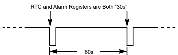
Figure 18. \overline{\text{IRQ}}/\text{F}_{\text{OUT}} Waveform
