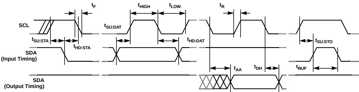
Figure 3. SDA vs SCL Timing
