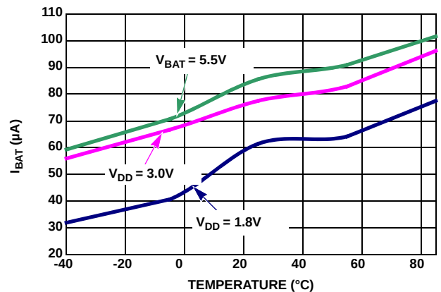
Figure 13. I_{BAT} with TSE = 1, BTSE = 1 vs Temperature
