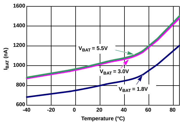
Figure 7. I_{BAT} vs Temperature ( V_{DD} = 0V )
