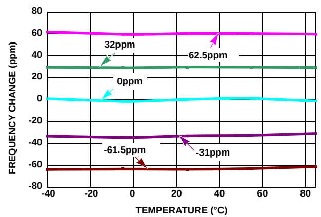
Figure 15. Oscillator Change vs Temperature at Different Aging Settings (IATR) (BETA Set for 1ppm Steps)
