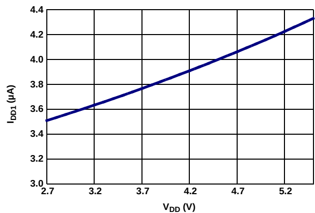
Figure 9. I_{DD1} vs V_{DD}
