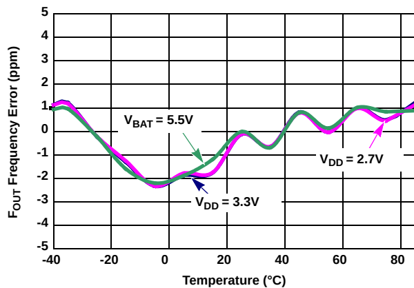
Figure 10. Oscillator Error vs Temperature
