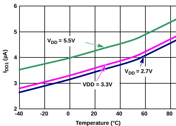
Figure 8. I_{DD1} vs Temperature
