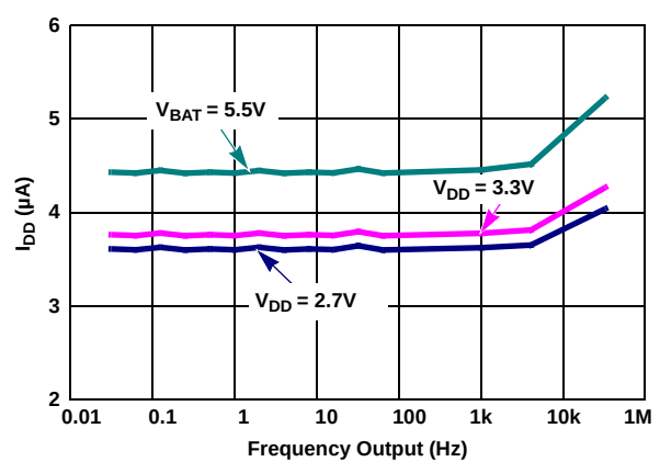
Figure 11. F_{OUT} vs I_{DD}
