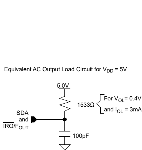
Figure 4. Standard Output Load for Testing the Device with V_{DD} = 5.0V
