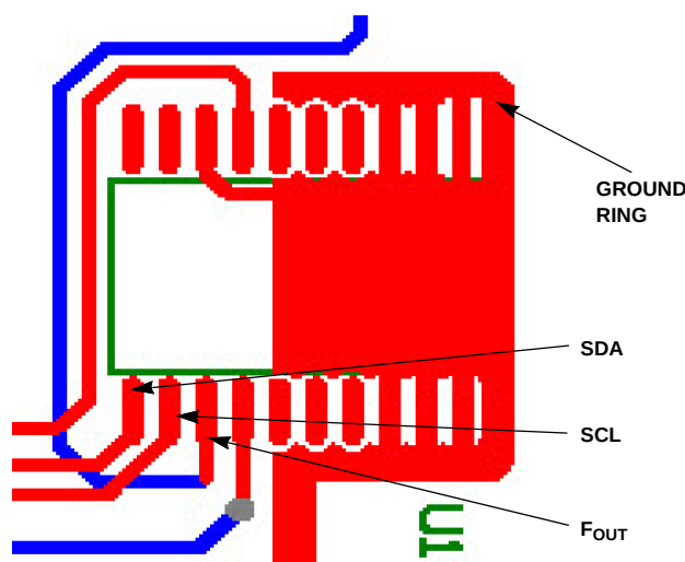
Figure 25. Suggested Layout for the ISL12022MA
