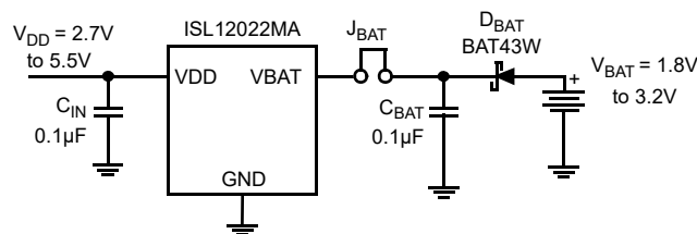
Figure 24. Suggested Battery Backup Circuit
