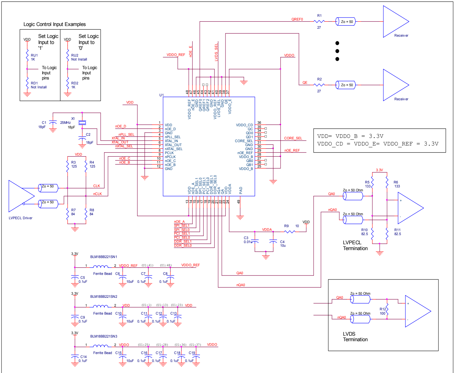
Figure 7. ICS8430S803I Schematic Example
