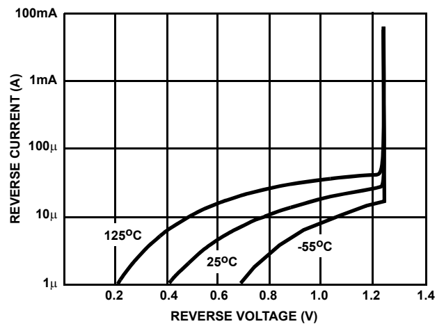
FIGURE 2. REVERSE VOLTAGE AS A FUNCTION OF CURRENT
