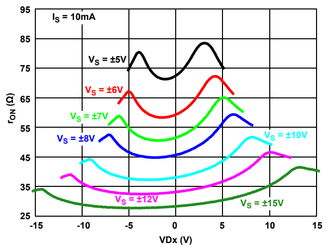
Figure 13. r_{ON} vs Signal Level vs Supply Voltages
