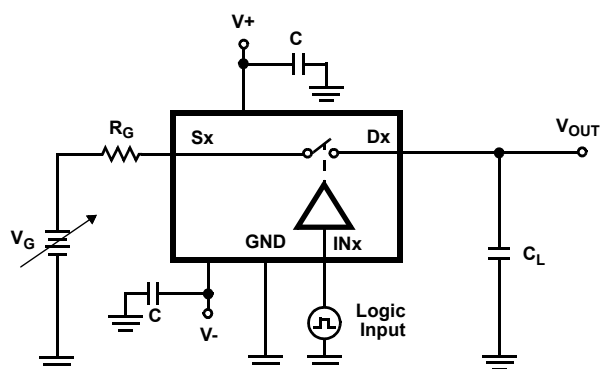
Figure 5. Switching Times Test Circuit
