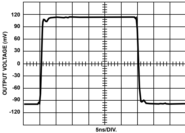
FIGURE 4. SMALL SIGNAL PULSE RESPONSE ( A_V = +2 )
