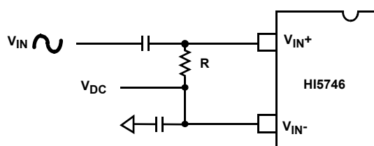
FIGURE 28. AC COUPLED SINGLE ENDED INPUT
