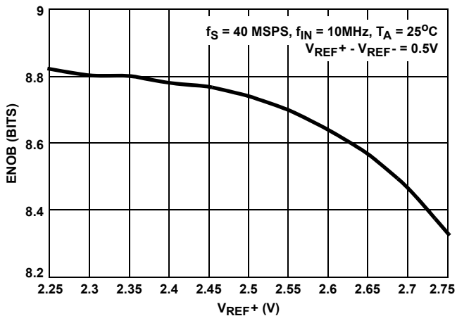
FIGURE 8. EFFECTIVE NUMBER OF BITS (ENOB) vs V_{REF+}
