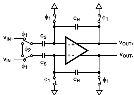
FIGURE 25. ANALOG INPUT SAMPLE-AND-HOLD
