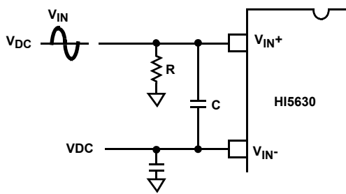
FIGURE 7. DC COUPLED SINGLE ENDED INPUT
