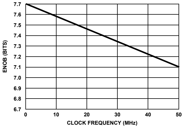
FIGURE 8. ENOB vs INPUT FREQUENCY ( f_{CLK} = 80MHz )
