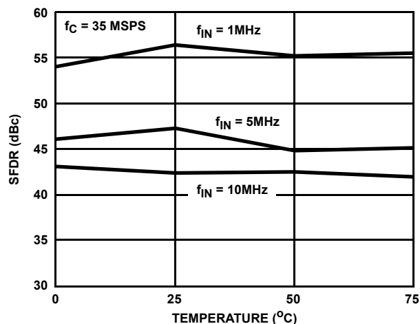
FIGURE 9. SFDR vs TEMPERATURE
