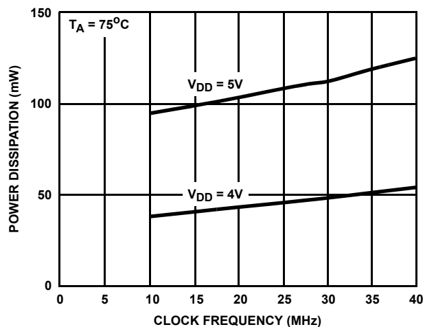
FIGURE 11. POWER DISSIPATION vs CLOCK FREQUENCY
