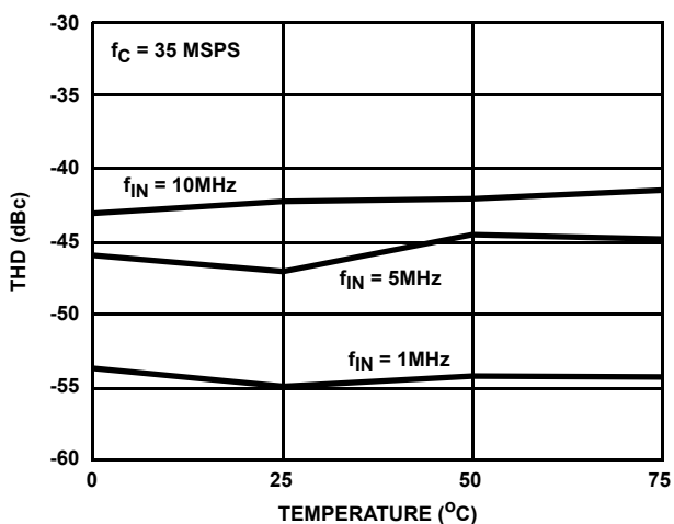
FIGURE 7. THD vs TEMPERATURE
