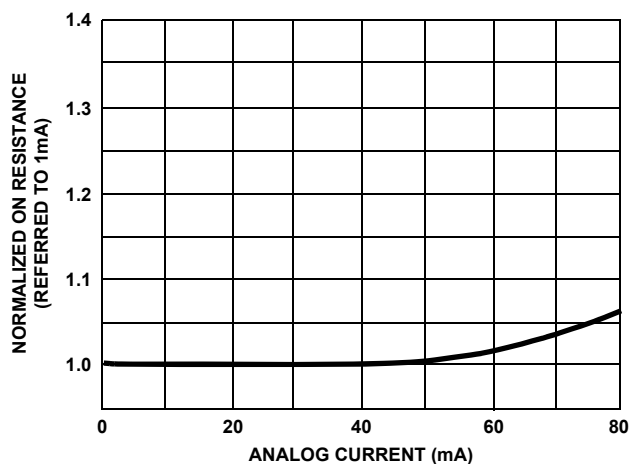
FIGURE 19. NORMALIZED ON RESISTANCE vs ANALOG CURRENT
