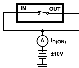
FIGURE 4. I_{D(ON)}
