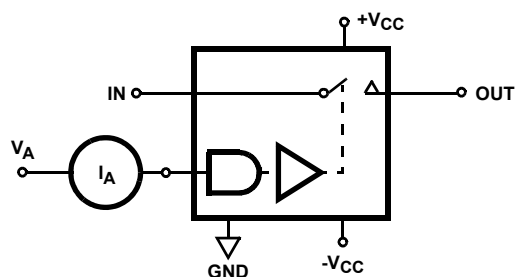
FIGURE 5. ADDRESS CURRENTS
