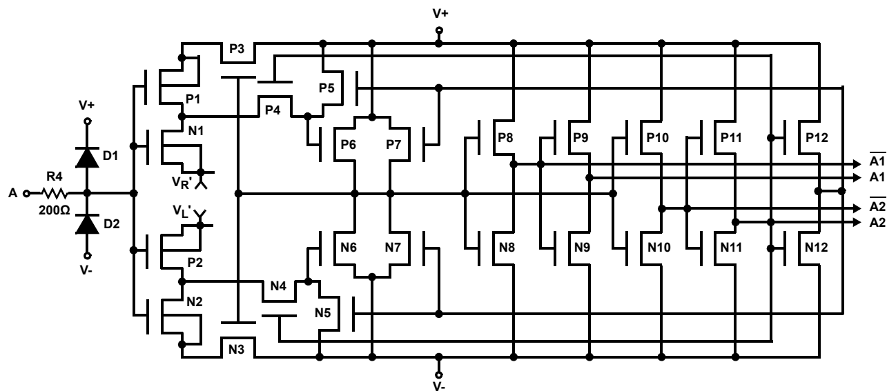
DIGITAL INPUT BUFFER AND LEVEL SHIFTER
