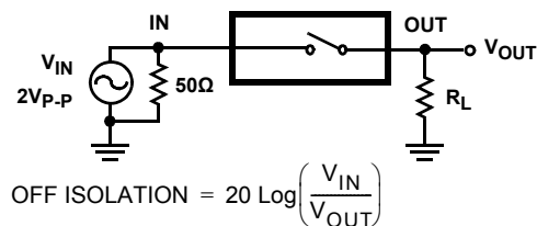
FIGURE 7. OFF ISOLATION
