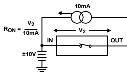
FIGURE 1. R_{DS}
