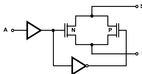
TYPICAL SWITCH
