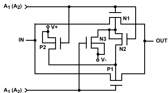
FIGURE 16. SWITCH CELL
