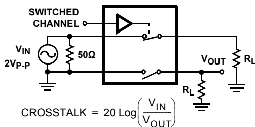
FIGURE 8. CROSSTALK
