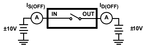
FIGURE 2. I_{S(OFF)}
