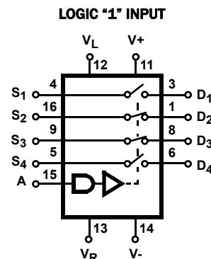
TYPICAL SWITCH
