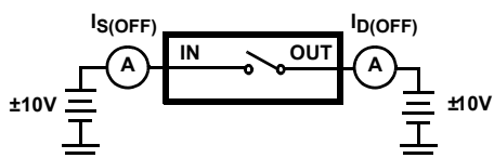
FIGURE 3. I_{D(OFF)}
