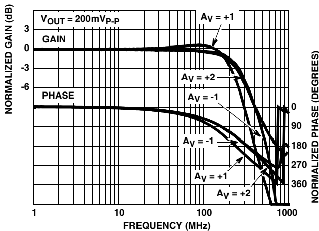
FIGURE 18. FREQUENCY RESPONSE
