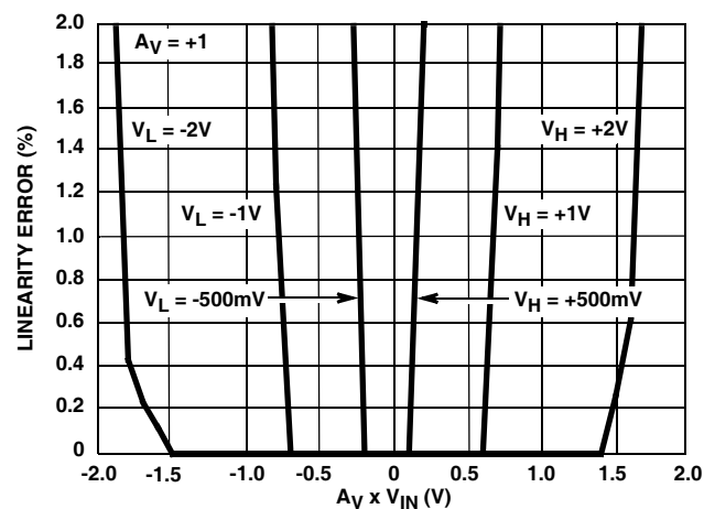
FIGURE 31. LINEARITY NEAR LIMIT VOLTAGE
