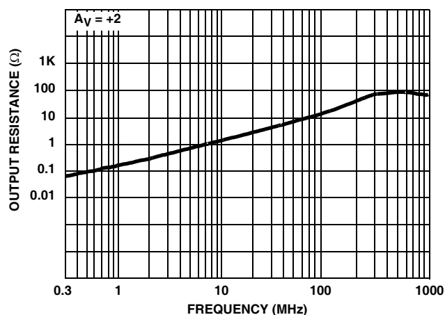
FIGURE 26. OUTPUT RESISTANCE
