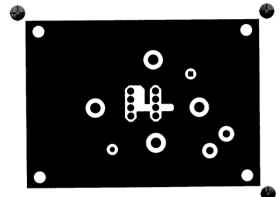
FIGURE 1C. BOTTOM LAYOUT
