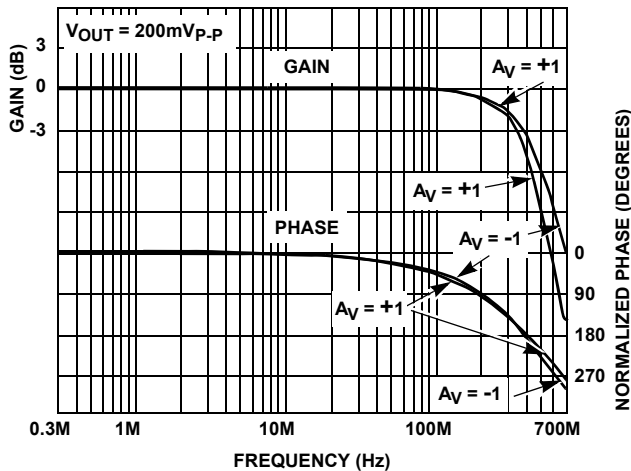
FIGURE 10. FREQUENCY RESPONSE
