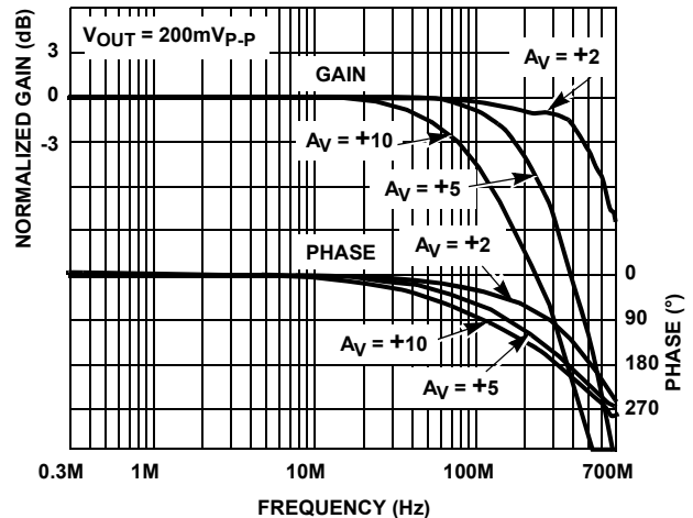
FIGURE 11. FREQUENCY RESPONSE
