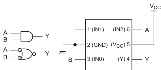
図 2. 2-inputs AND Gate
