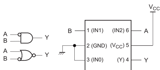
図 4. 2-inputs AND Gate with A input inverted
