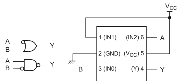
図 3. 2-inputs OR Gate with A input inverted
