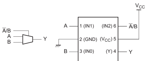
図 1. 2 to 1 Data Selector
