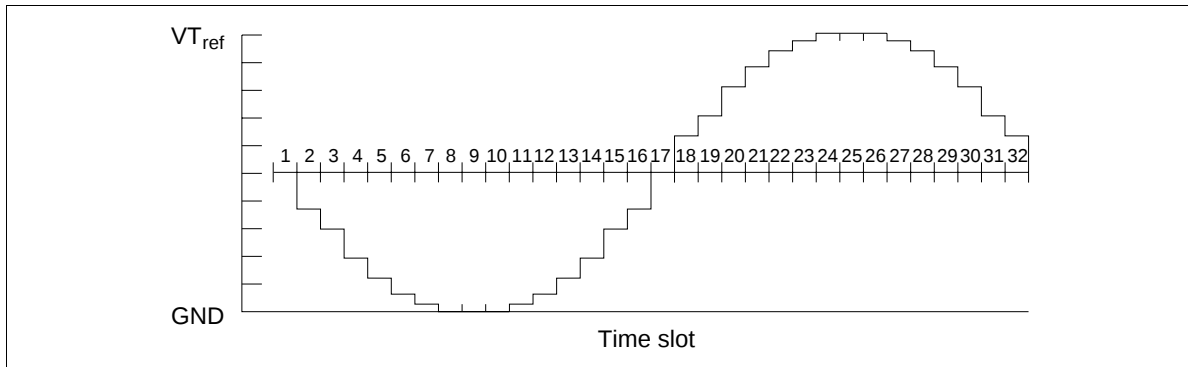
Figure 70 Waveform of Tone Output
