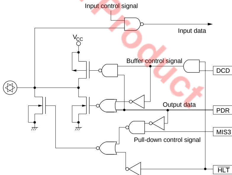
Figure 22 I/O Buffer Configuration (with Pull-Down MOS)
