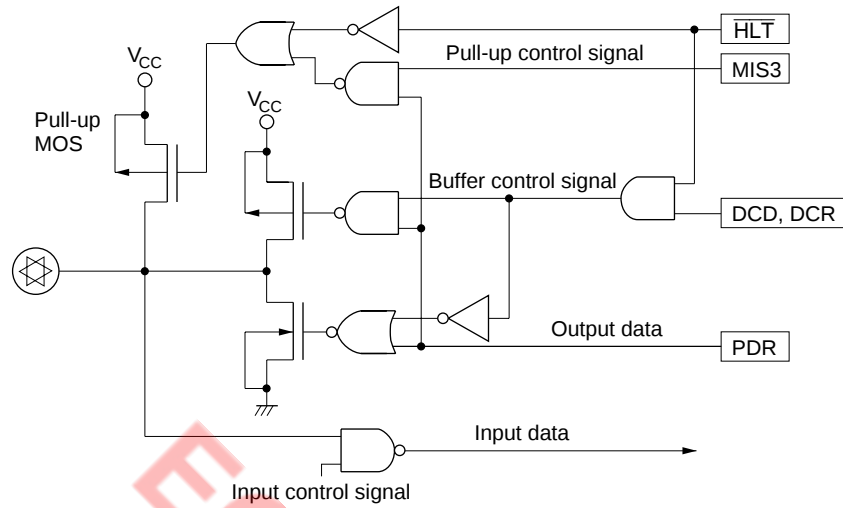
Figure 21 I/O Buffer Configuration (with Pull-Up MOS)
