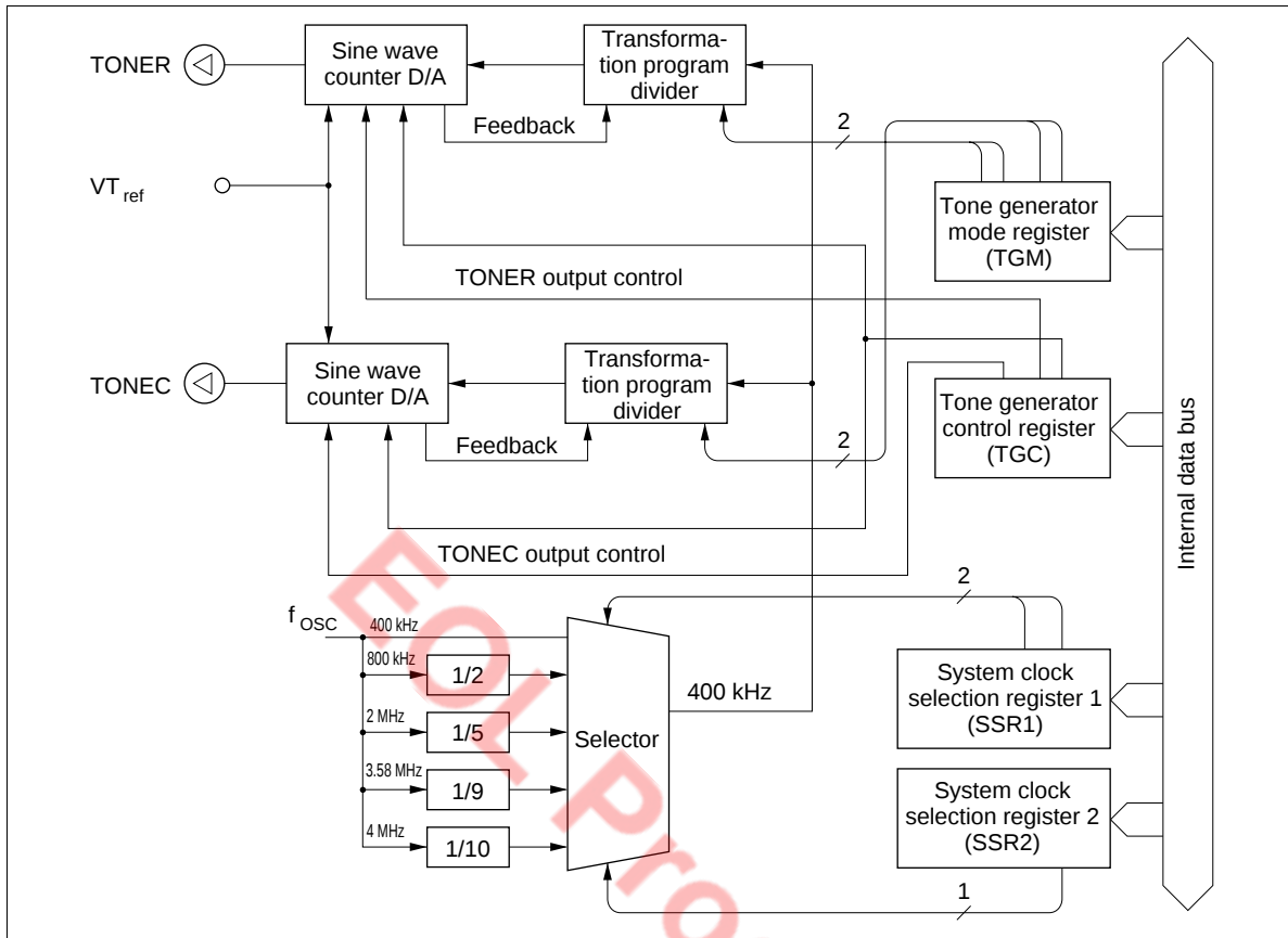
Figure 64 Block Diagram of DTMF Generator Circuit
