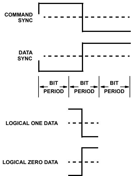
FIGURE 8. MIL-STD-1553 CHARACTER FORMATS
