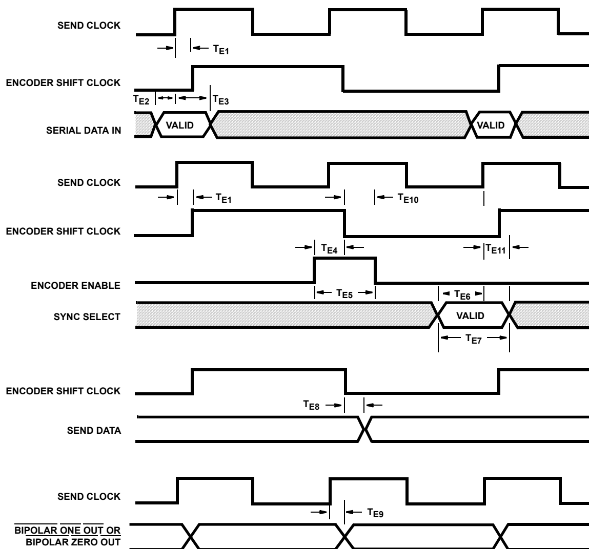
FIGURE 10. ENCODER TIMING
