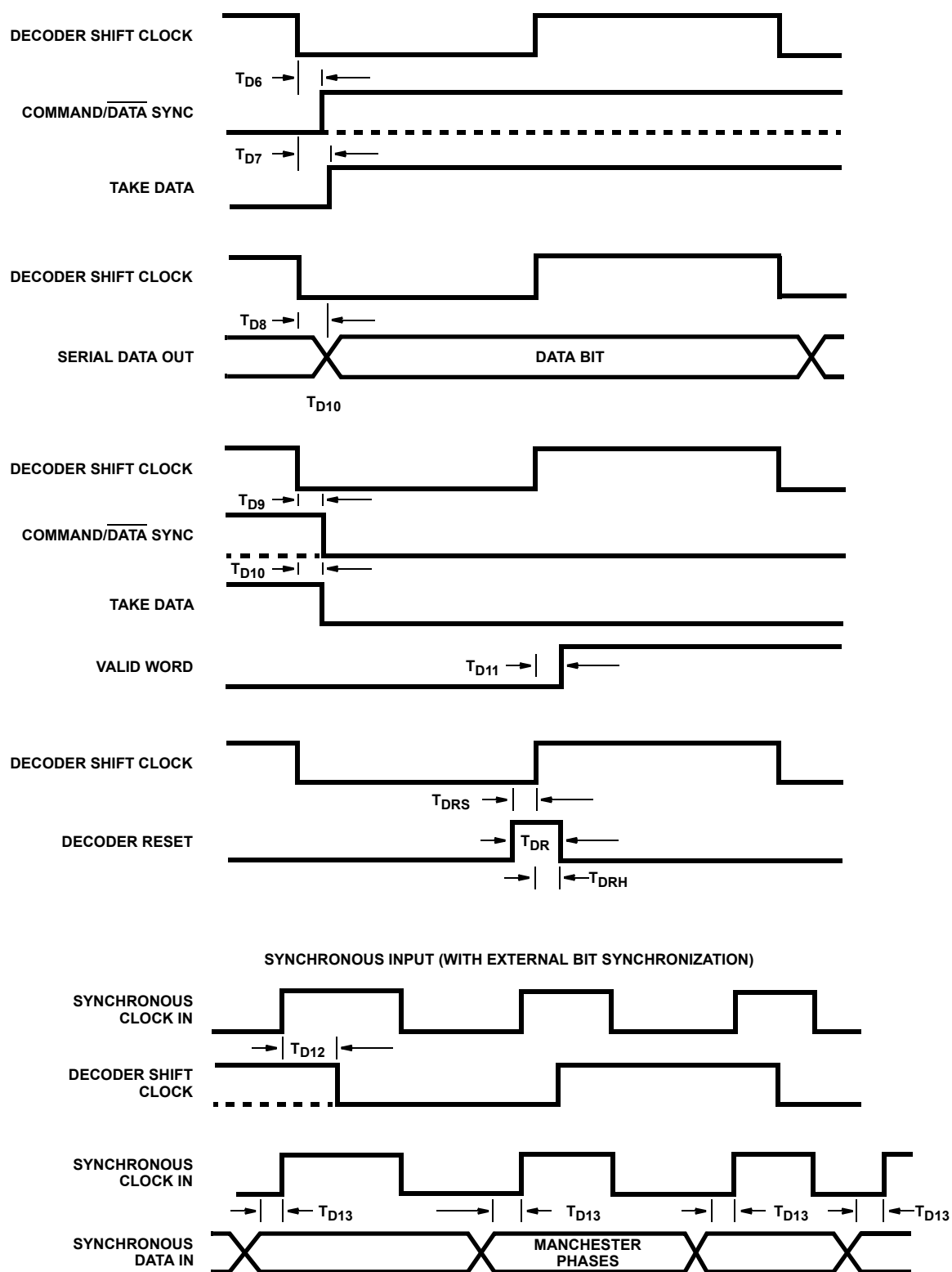
FIGURE 12. DECODER TIMINGS
