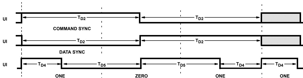
FIGURE 11. DECODER TIMING
