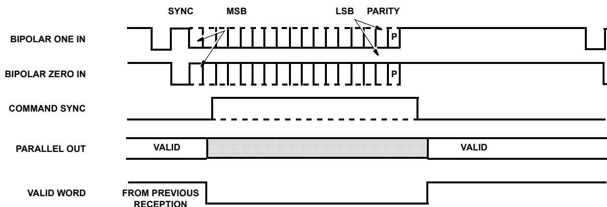
FIGURE 5. DECODER TIMING
