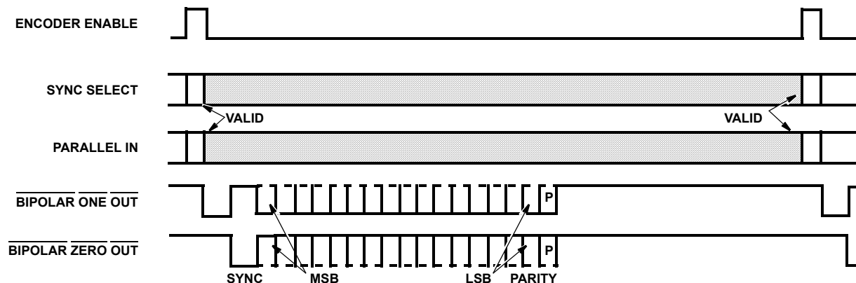
FIGURE 4. ENCODER TIMING
