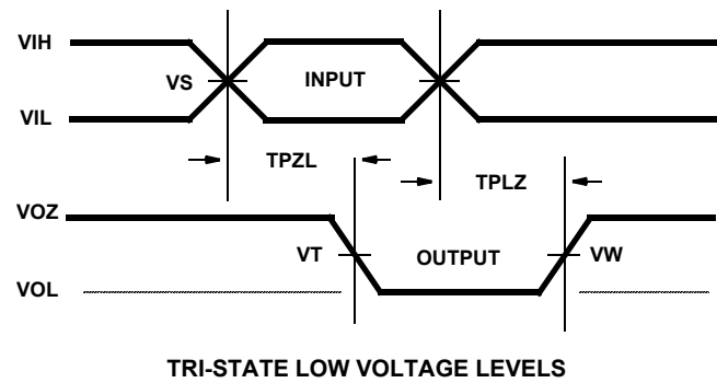
TRI-STATE LOW VOLTAGE LEVELS
