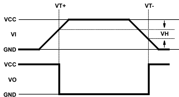
HYSTERESIS DEFINITION
