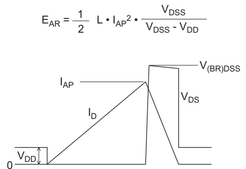
Avalanche Waveform
