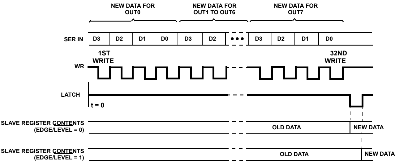
FIGURE 10. SERIAL PROGRAMMING MODE OPERATION (SER/PAR = 1)
