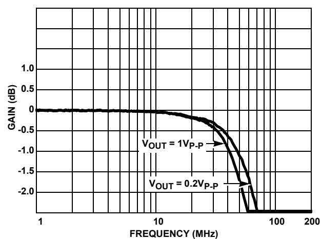
FIGURE 14. GAIN FLATNESS
