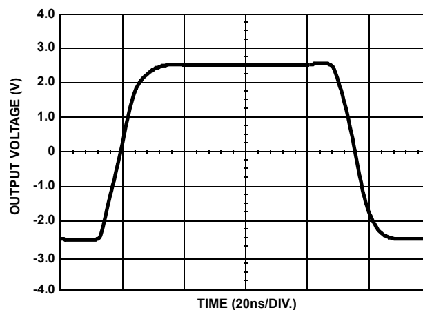
FIGURE 12. LARGE SIGNAL PULSE RESPONSE
