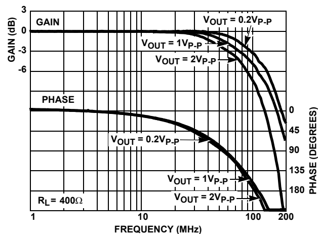
FIGURE 15. FREQUENCY RESPONSE
