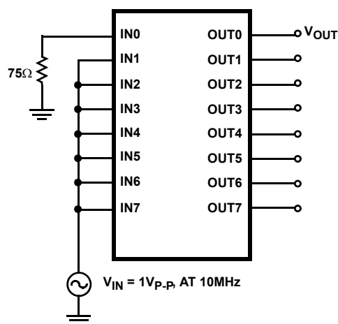
FIGURE 4. ALL HOSTILE CROSSTALK (NOTES 10, 15, 17-19)
