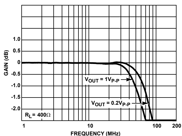
FIGURE 16. GAIN FLATNESS
