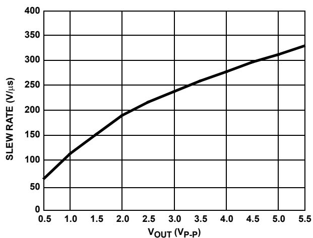
FIGURE 19. SLEW RATE vs V_{\text{OUT}}
