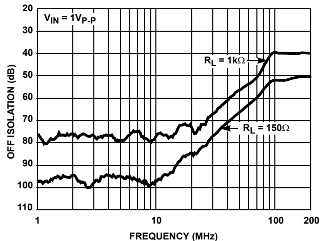
FIGURE 18. ALL HOSTILE OFF-ISOLATION
