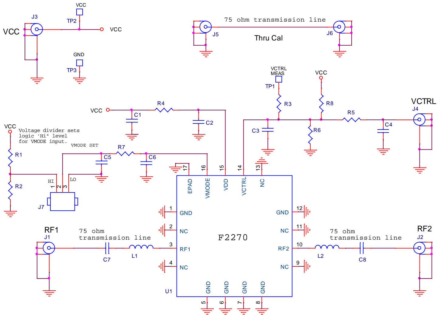
Figure 60. Electrical Schematic
