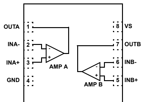
EL1509 (8 LD DFN) TOP VIEW
