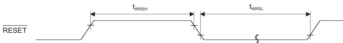
Figure 4-3: \overline{\text{RESET}} timing
