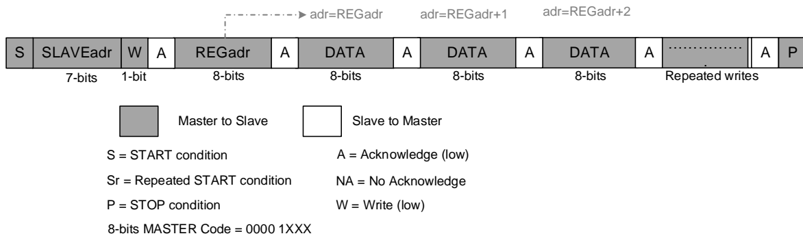
Figure 18: Consecutive Write Command
