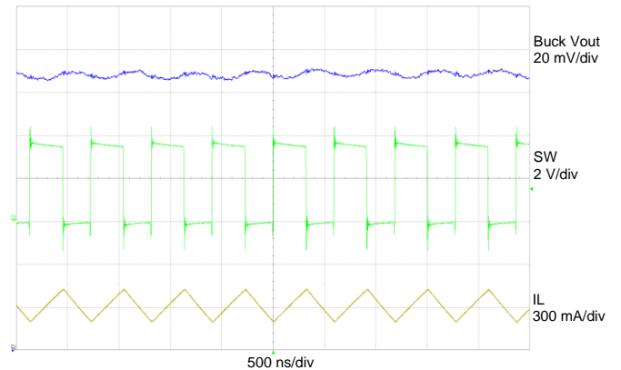
Figure 28: Buck V_{IN} = 3.6\text{ V} , Buck V_{OUT} = 1.8\text{ V} , Buck I_{LOAD} = 300\text{ mA}
