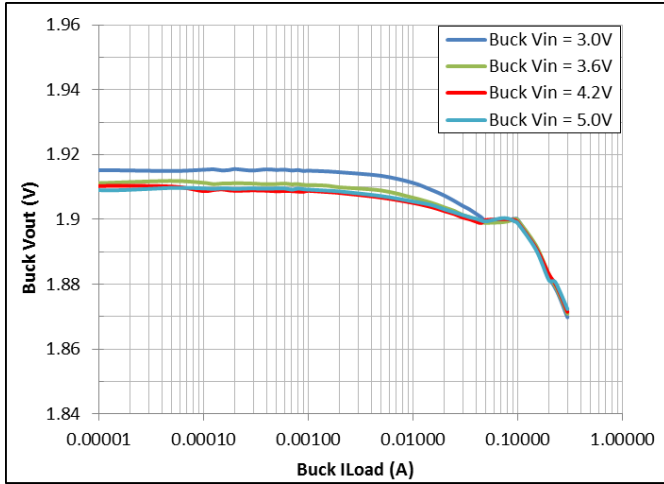
Figure 21: Buck V_{OUT} = 1.9 V
