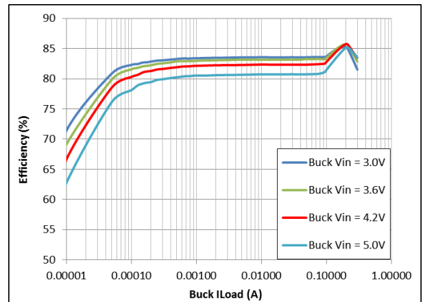
Figure 11: Buck V_{OUT} = 0.9\text{ V}
