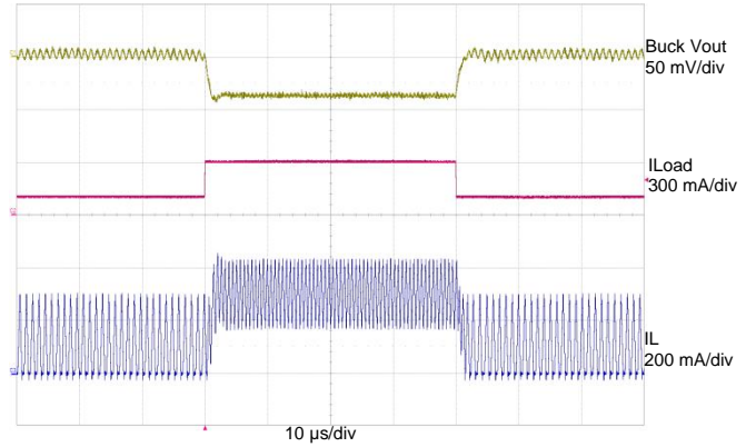
Figure 30: Buck I_{LOAD} = 100\text{ mA} to 300\text{ mA} to 100\text{ mA} ( 0.2\text{ A}/\mu\text{s} ); Buck V_{IN} = 3.6\text{ V} , Buck V_{OUT} = 1.8\text{ V}
