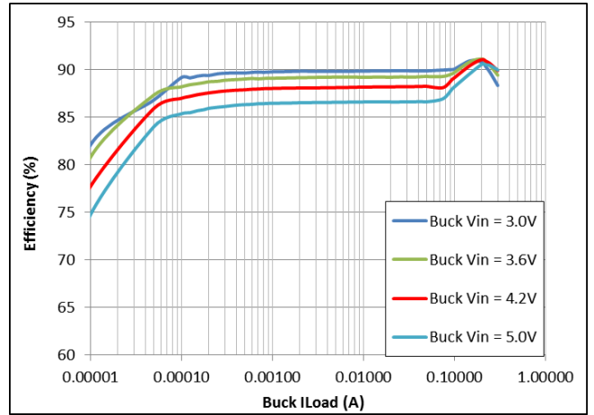
Figure 9: Buck V_{OUT} = 1.8\text{ V}
