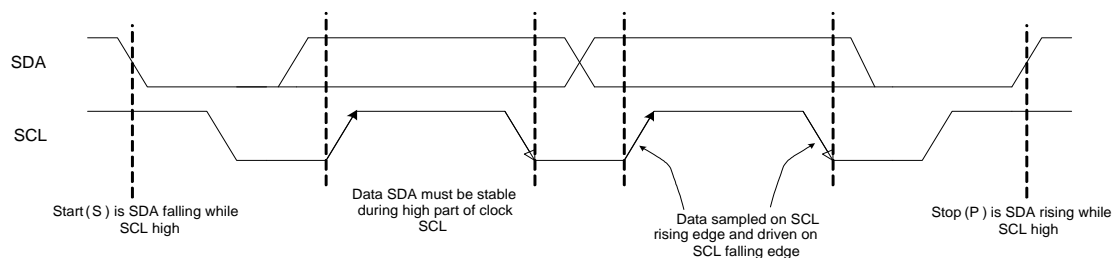
Figure 44: I 2 C Start and Stop Conditions
