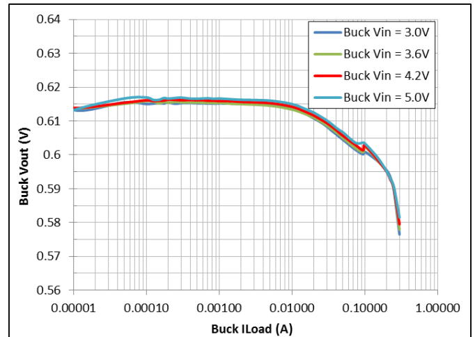
Figure 24: Buck V_{OUT} = 0.6 V
