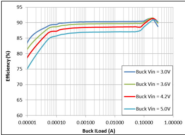
Figure 8: Buck V_{OUT} = 1.9\text{ V}
