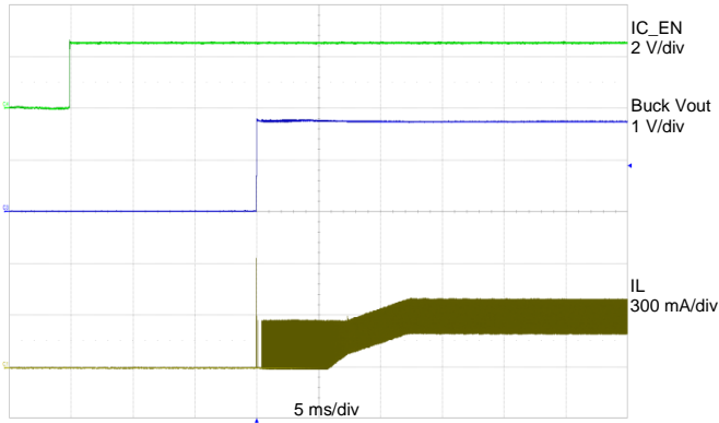
Figure 41: Device Enable: Buck V_{IN} = 3.6\text{ V} , Buck V_{OUT} 1.8\text{ V} , Buck I_{LOAD} = 300\text{ mA}
