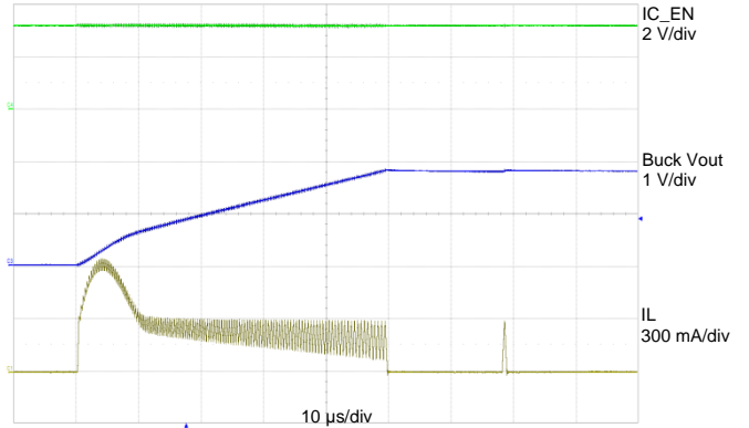
Figure 42: V_{OUT} Ramp-Up after Enabled (Zoom-in of Figure 41 )
