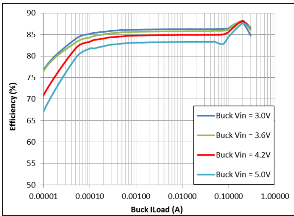
Figure 10: Buck V_{OUT} = 1.2\text{ V}
