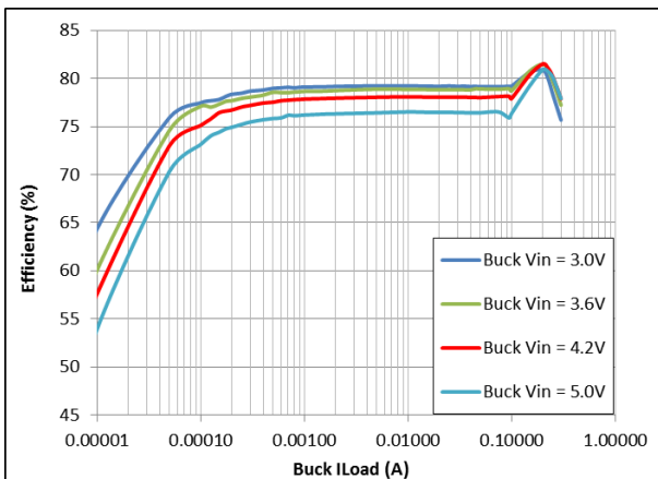
Figure 12: Buck V_{OUT} = 0.6\text{ V}
