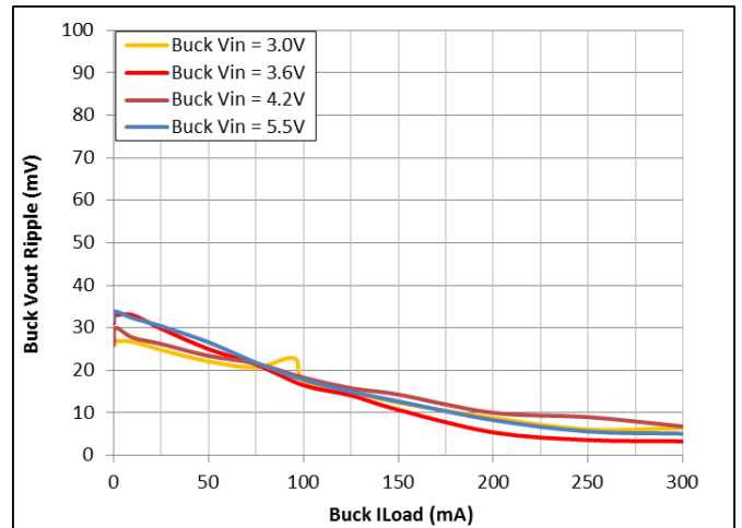
Figure 20: Buck V_{OUT} = 0.6 V
