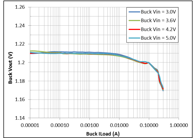
Figure 22: Buck V_{OUT} = 1.2 V
