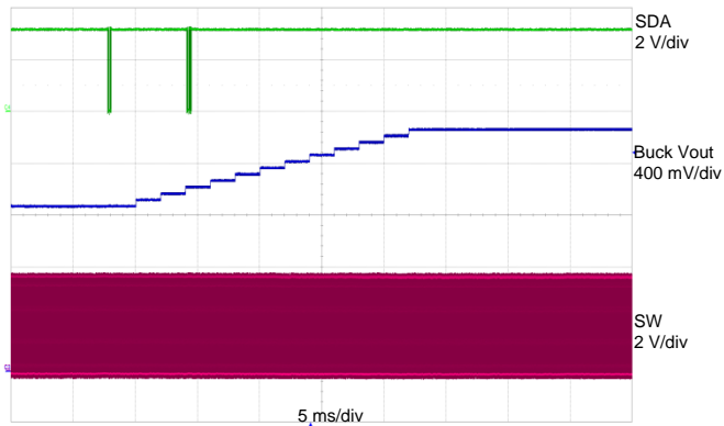
Figure 39: Buck V OUT 1.3 V to 1.9 V; Buck V IN = 3.6 V, Buck I LOAD = 300 mA
