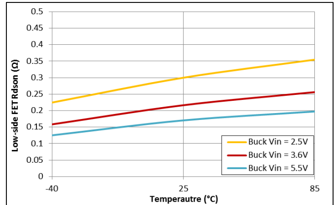
Figure 7: Low-Side FET
