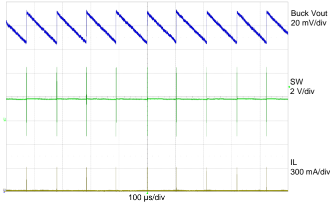
Figure 25: Buck V_{IN} = 3.6\text{ V} , Buck V_{OUT} = 1.8\text{ V} , Buck I_{LOAD} = 1\text{ mA}
