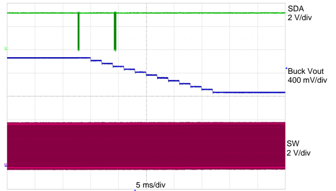
Figure 40: Buck V OUT 1.9 V to 1.3 V; Buck V IN = 3.6 V, Buck I LOAD = 300 mA
