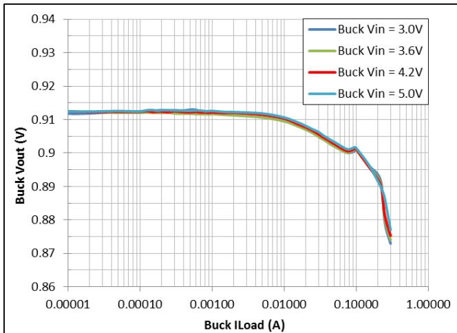
Figure 23: Buck V_{OUT} = 0.9 V
