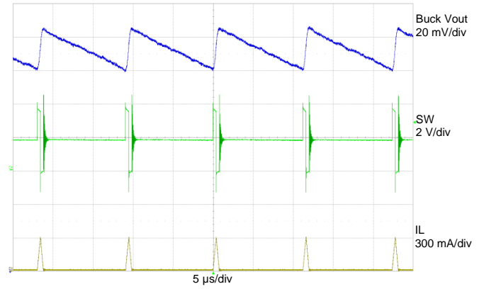
Figure 26: Buck V_{IN} = 3.6\text{ V} , Buck V_{OUT} = 1.8\text{ V} , Buck I_{LOAD} = 10\text{ mA}
