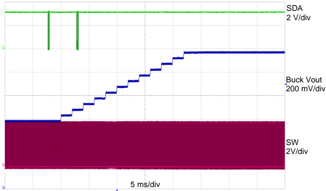
Figure 37: Buck V OUT 0.6 V to 1.2 V; Buck V IN = 3.6 V, Buck I LOAD = 300 mA
