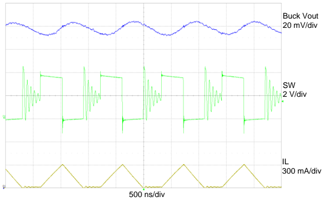
Figure 27: Buck V_{IN} = 3.6\text{ V} , Buck V_{OUT} = 1.8\text{ V} , Buck I_{LOAD} = 100\text{ mA}
