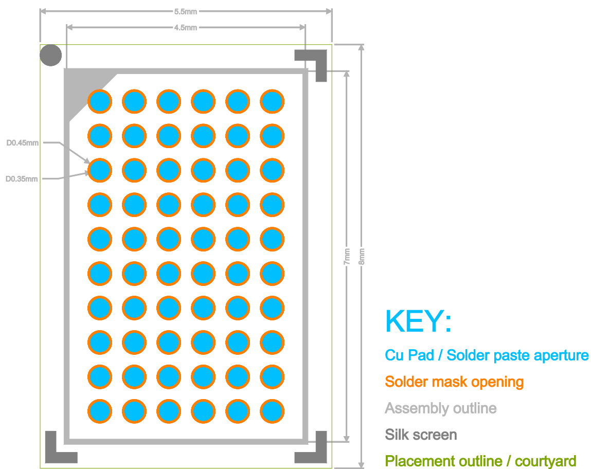
Figure 14. DA9141-A Footprint
