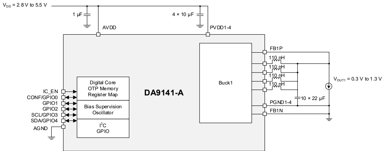
Figure 1. Block Diagram
